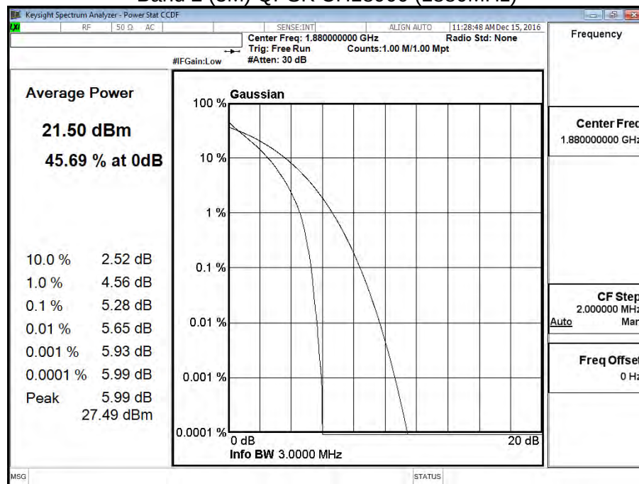
Band 2 (3M) QPSK CH18900 (1880MHz)
