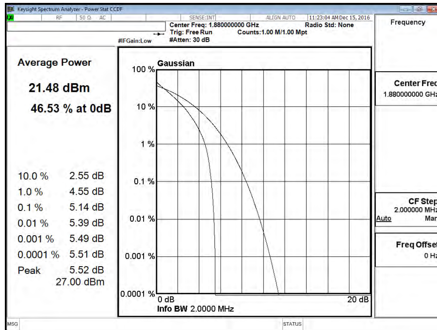
Band 2 (1.4M) QPSK CH18900 (1880MHz)
