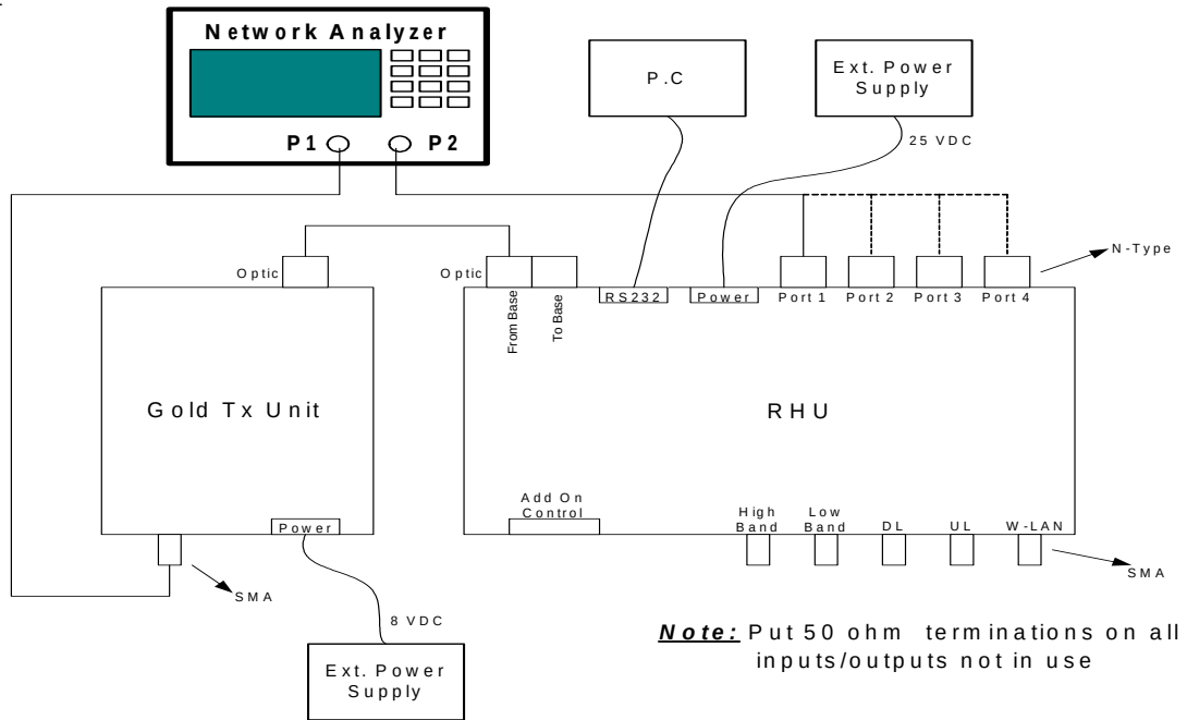
Figure 4.1: Network Analyzer DL
