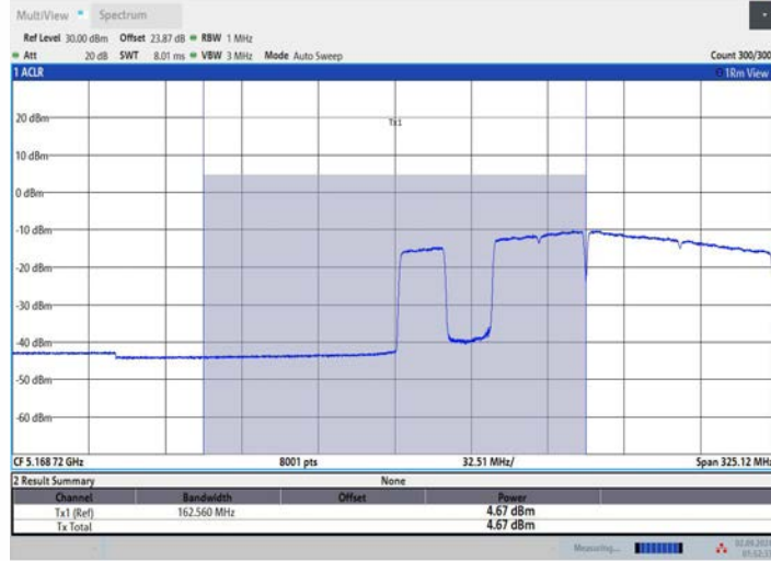
11BE160MIMO_Ant3_5250_UNII-1_996+484+242_OFDMA_2
