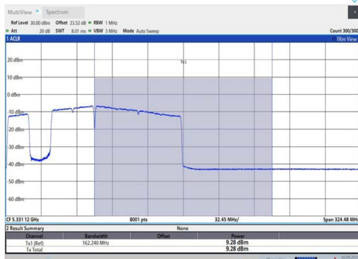
11BE160MIMO Ant1 5250 UNII-2A 996+484+242 OFDMA 3
