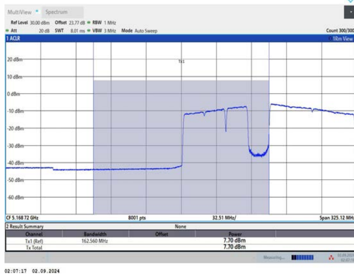
11BE160MIMO_Ant1_5250_UNII-1_996+484+242_OFDMA_5
