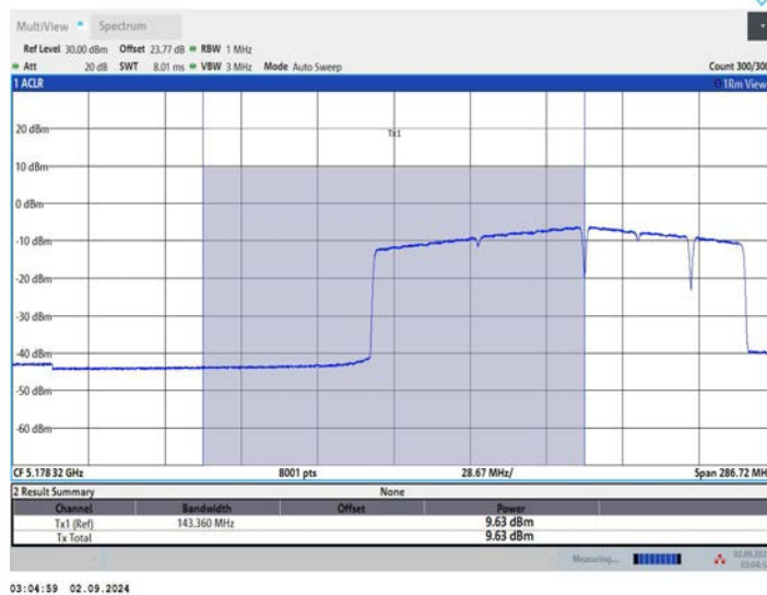
11BE160MIMO_Ant2_5250_UNII-1_996+484+242_OFDMA_1
