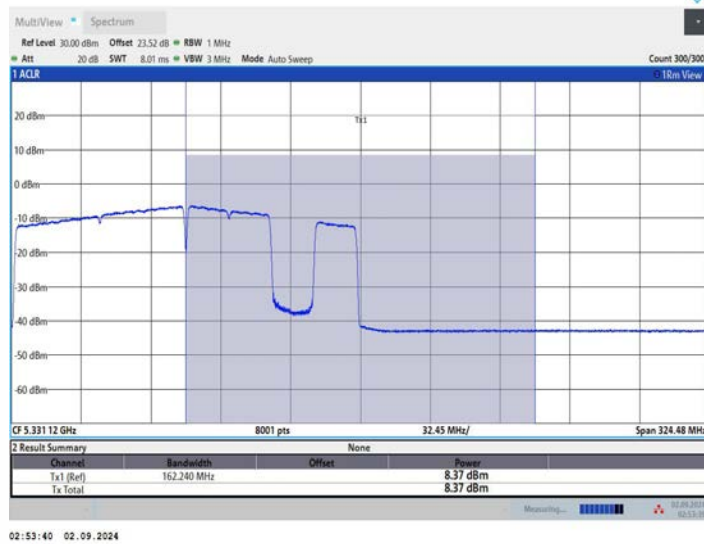
11BE160MIMO Ant1 5250 UNII-2A 996+484+242 OFDMA 8
