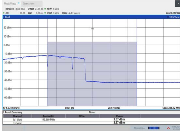
11BE160MIMO Ant2 5250 UNII-2A 996+484+242 OFDMA 8
