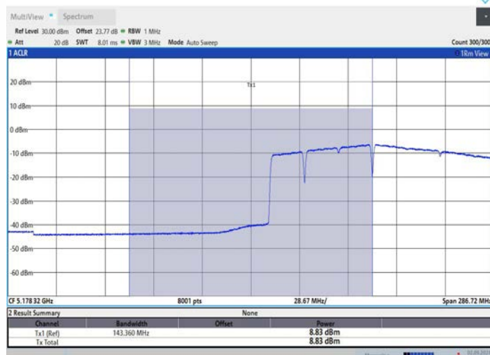
11BE160MIMO_Ant1_5250_UNII-1_996+484+242_OFDMA_2
