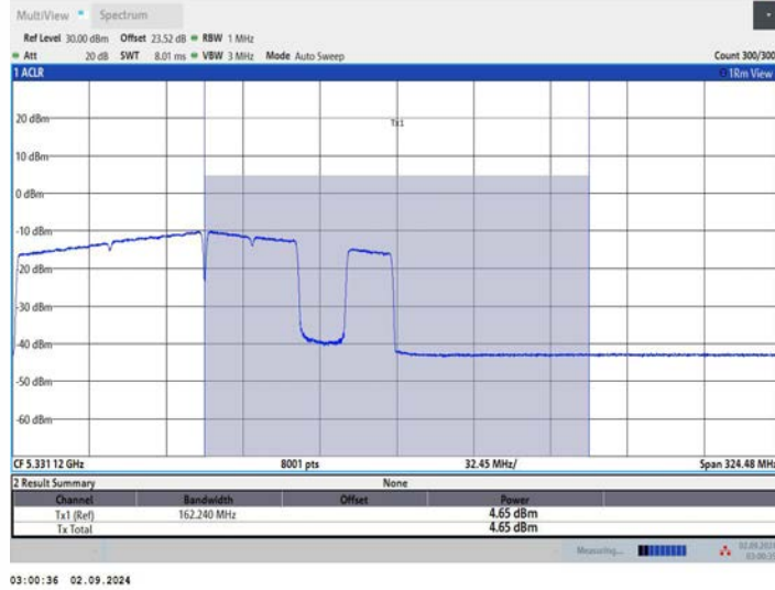
11BE160MIMO Ant1 5250 UNII-2A 996+484+242 OFDMA 7
