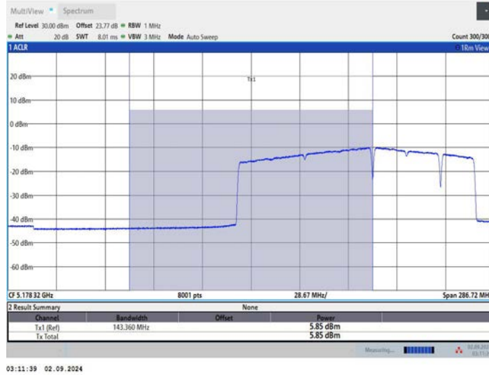
11BE160MIMO_Ant1_5250_UNII-1_996+484+242_OFDMA_8
