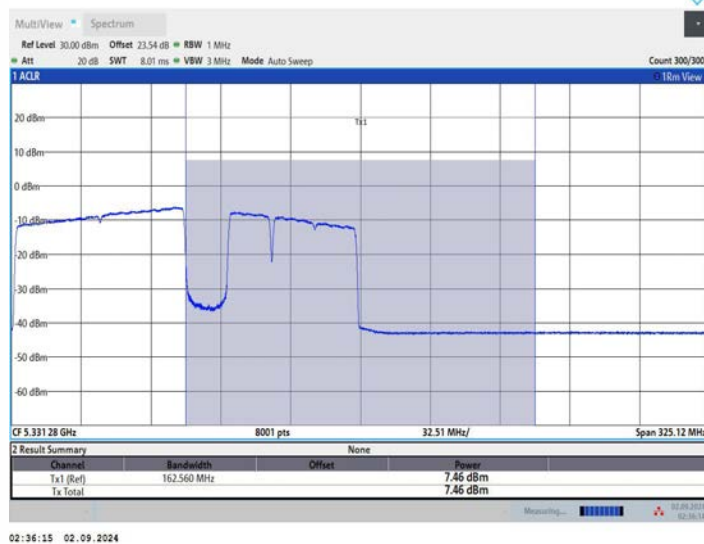
11BE160MIMO_Ant3_5250_UNII-2A_996+484+242_OFDMA_6
