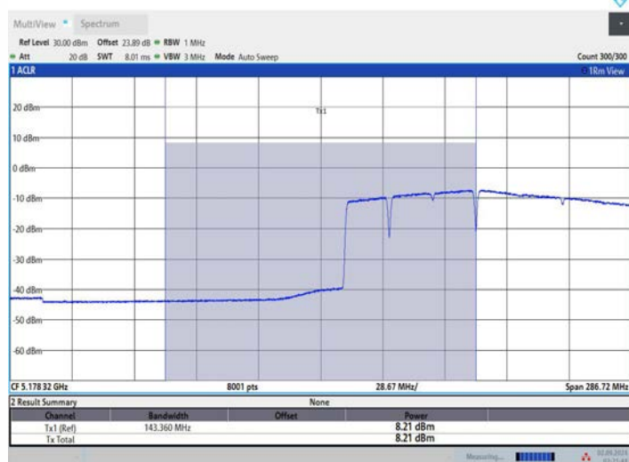
11BE160MIMO_Ant2_5250_UNII-1_996+484+242_OFDMA_2
