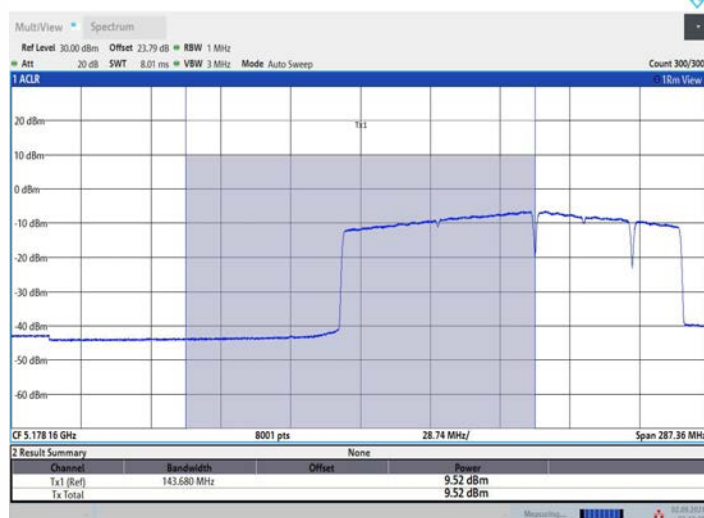
11BE160MIMO_Ant1_5250_UNII-2A_996+484+242_OFDMA_1
