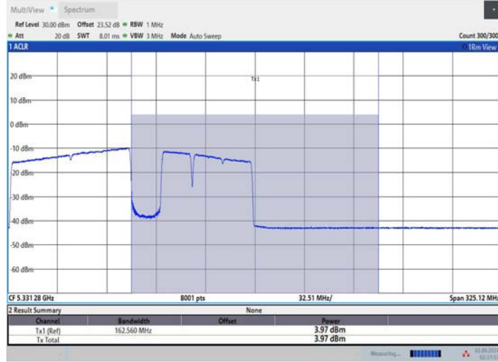
11BE160MIMO Ant1 5250 UNII-2A 996+484+242 OFDMA 5
