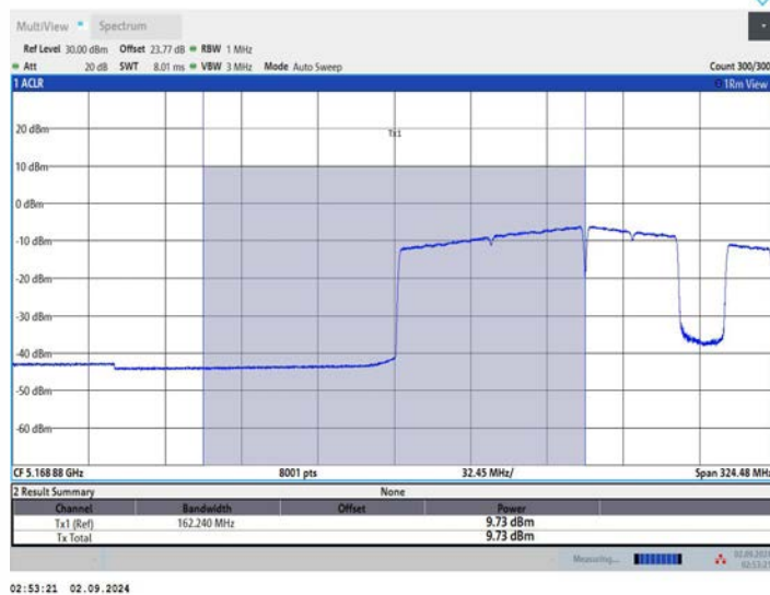
11BE160MIMO_Ant1_5250_UNII-1_996+484+242_OFDMA_8
