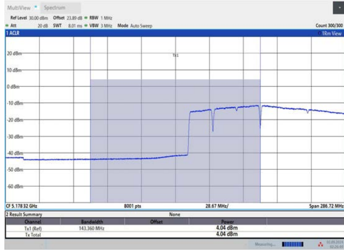
11BE160MIMO_Ant2_5250_UNII-1_996+484+242_OFDMA_1
