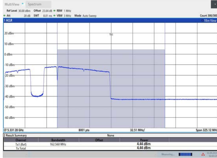
11BE160MIMO_Ant2_5250_UNII-2A_996+484+242_OFDMA_3
