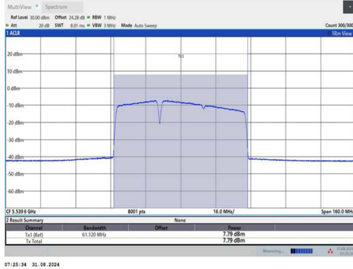
11BE80MIMO_Ant1_5530_484+242_OFDMA_1
