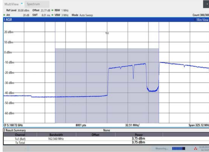
11BE160MIMO_Ant1_5250_UNII-1_996+484+242_OFDMA_4
