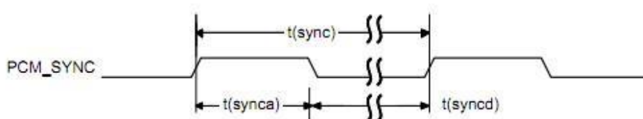
Figure 5- 14 PCM_SYNC Timing
