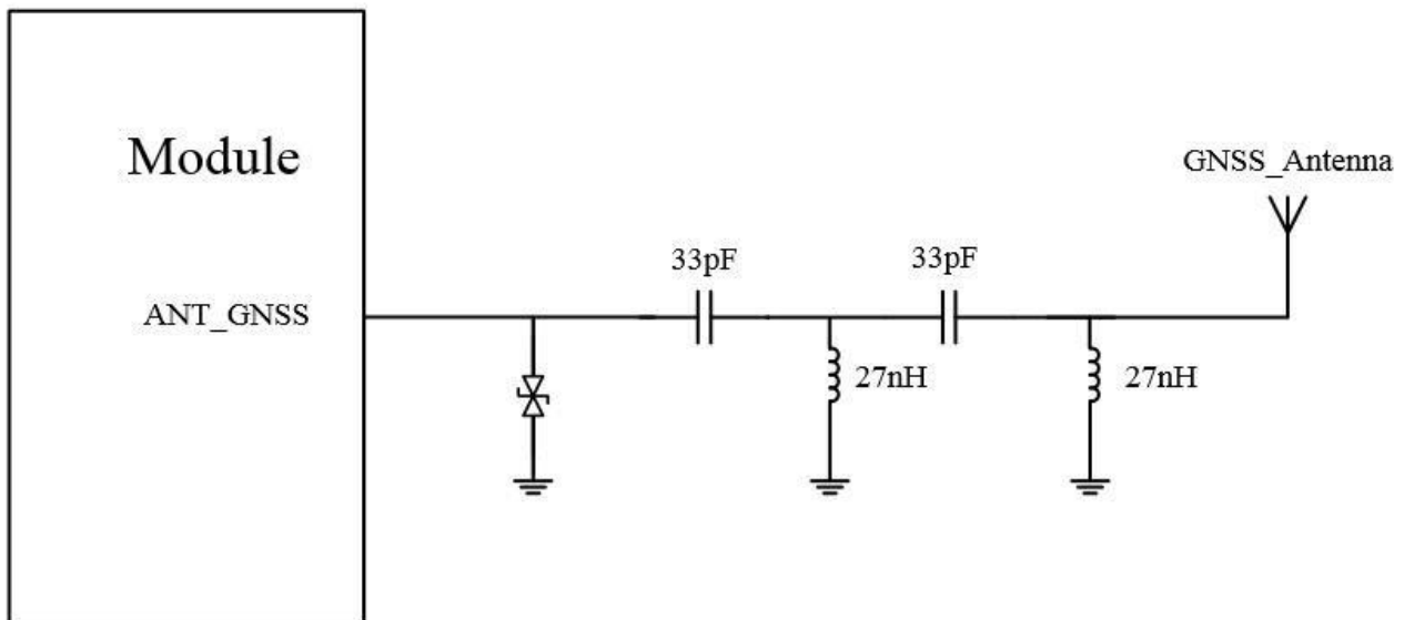
Figure 7- 2 GNSS Antenna Reference Circuit
