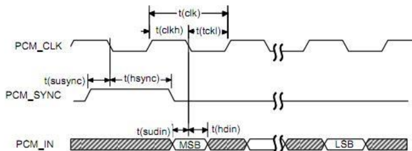
Figure 5- 15 PCM_CODEC to NL668-LA Timing
