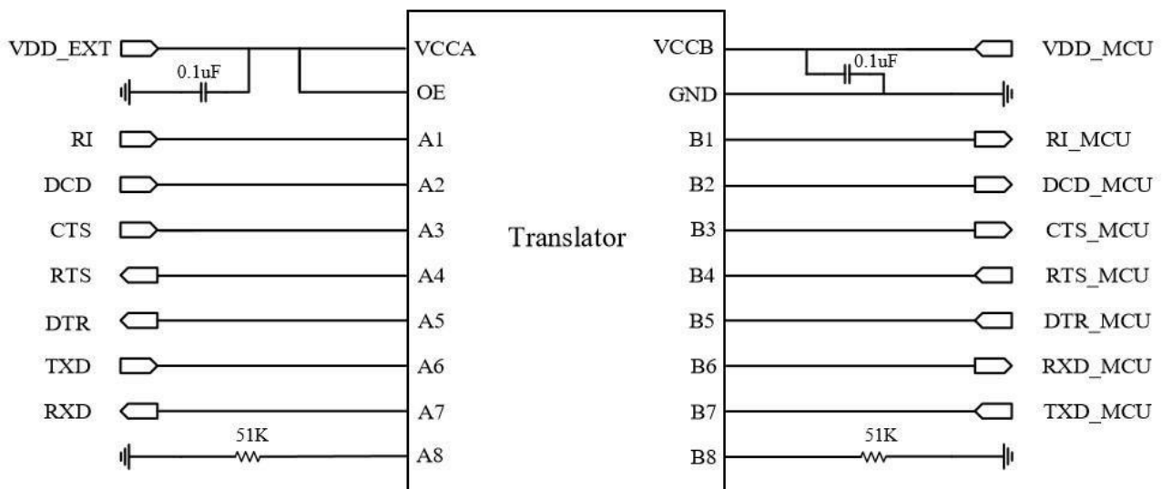
Figure 5- 12 UART Level Translate Reference 1
