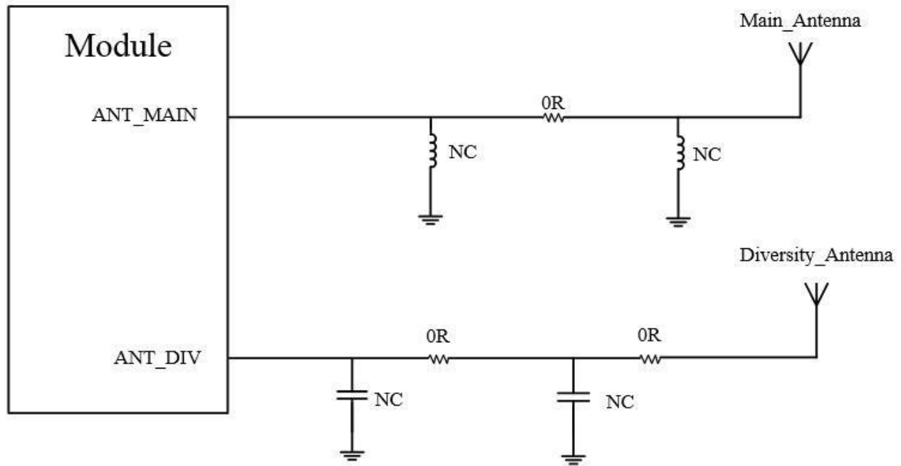
Figure 7- 1 Main and diversity Antenna Reference Circuit
