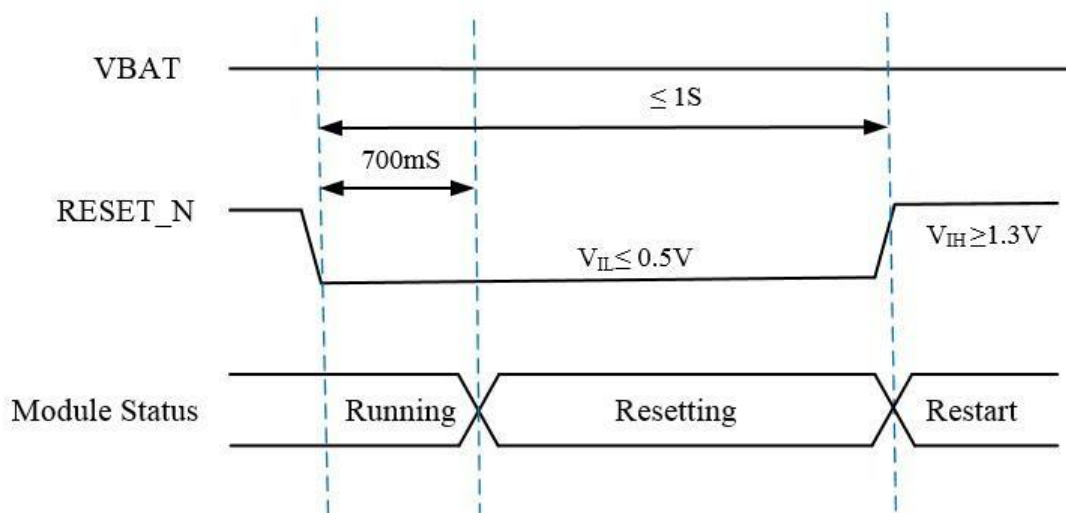
Figure 5- 7 Reset Timing
