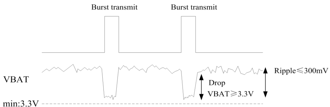
Figure 4- 2 Power Limit
