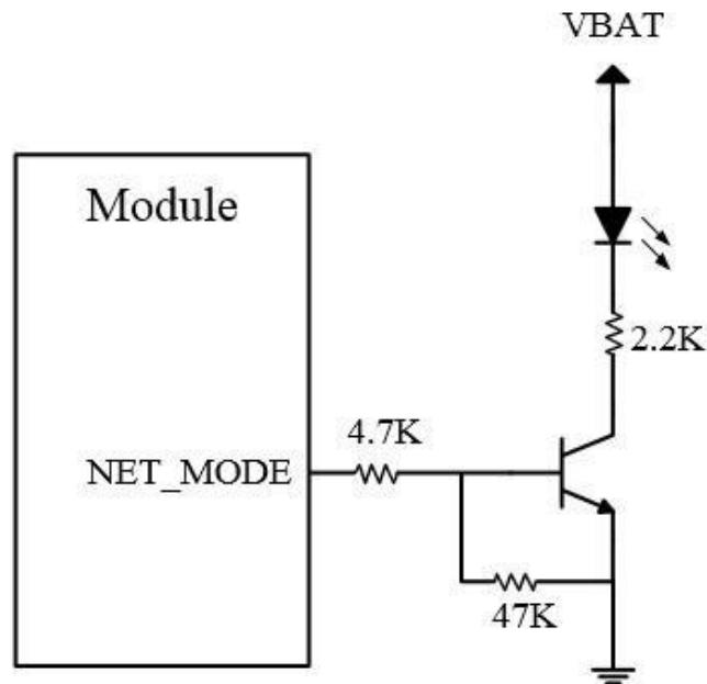
Figure 5- 8 Network Indicate Light Reference Circuits
