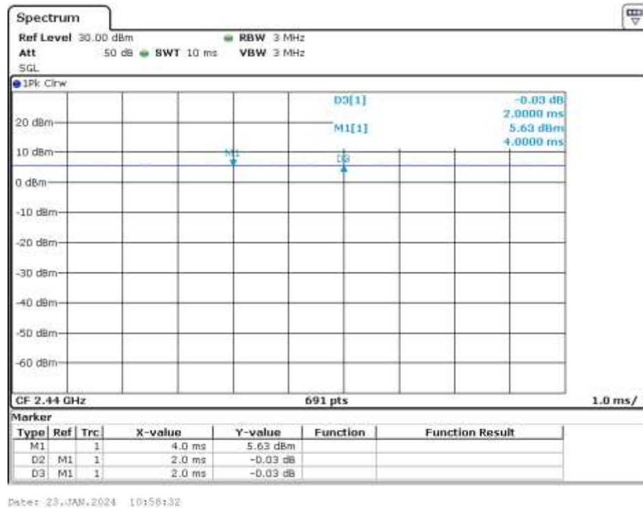
Figure 8-1 Bluetooth Transmission Plot
