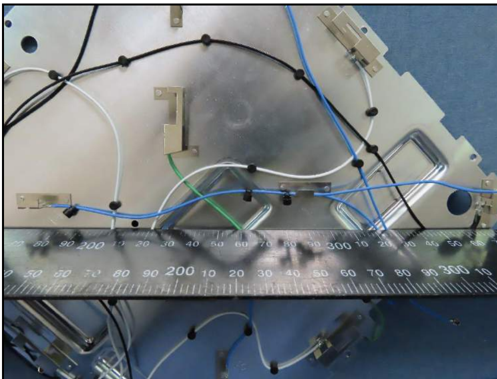
Antenna NO. 14
