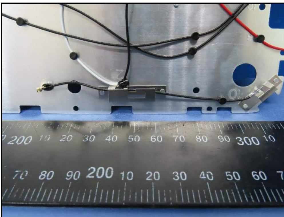
Antenna NO. 10
