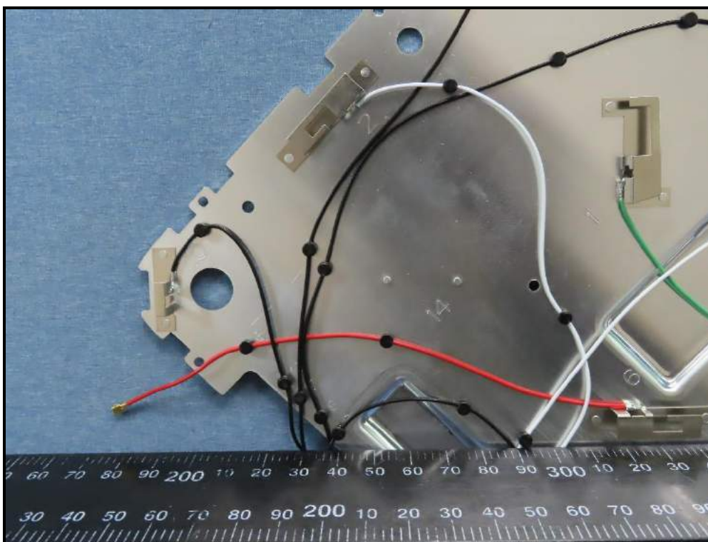
Antenna NO. 6
