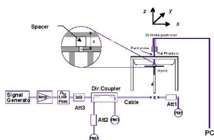
Figure 4-1 System Verification Setup Diagram
