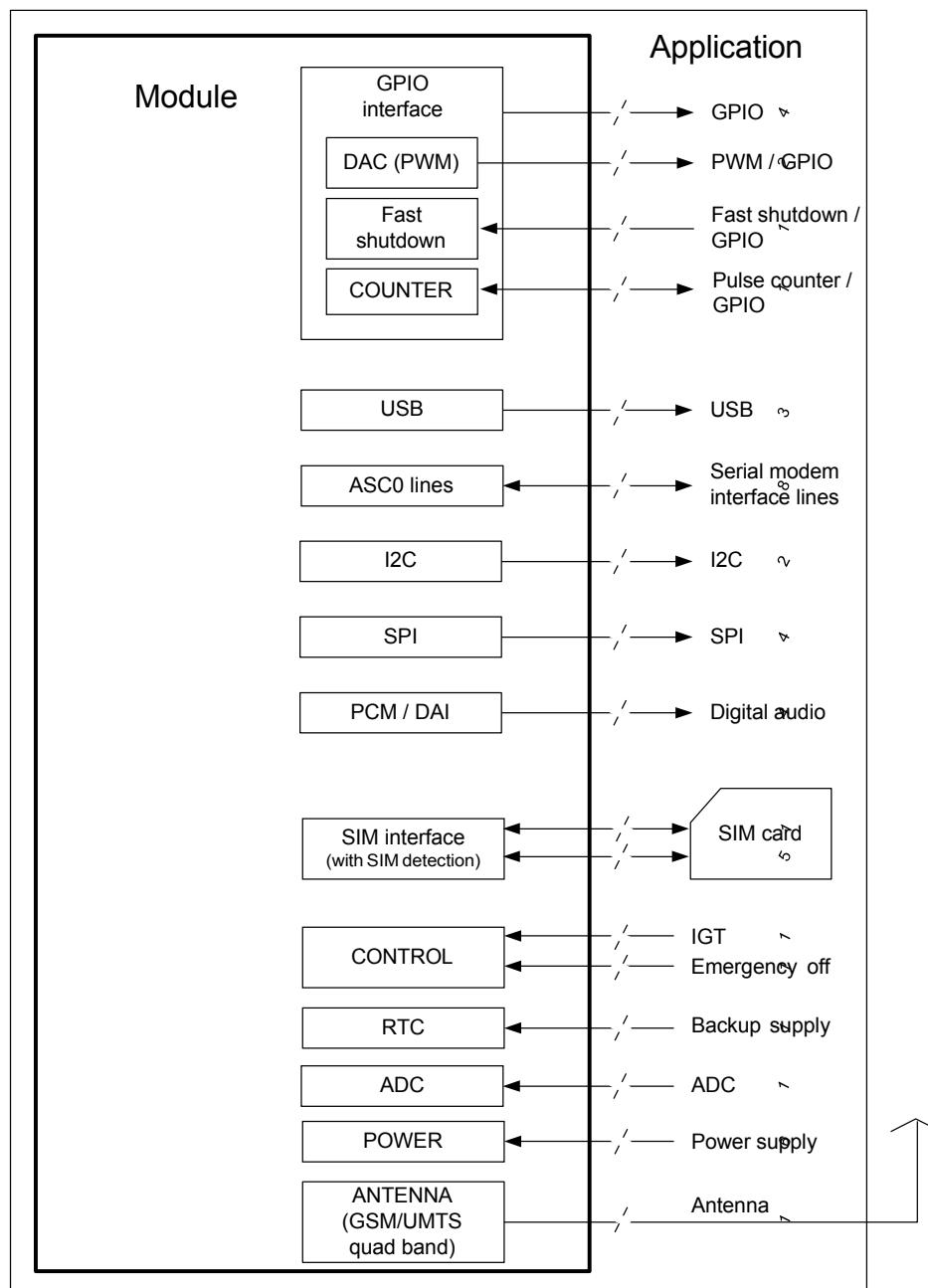
Figure 1: PDS5-E/PDS5-US system overview
