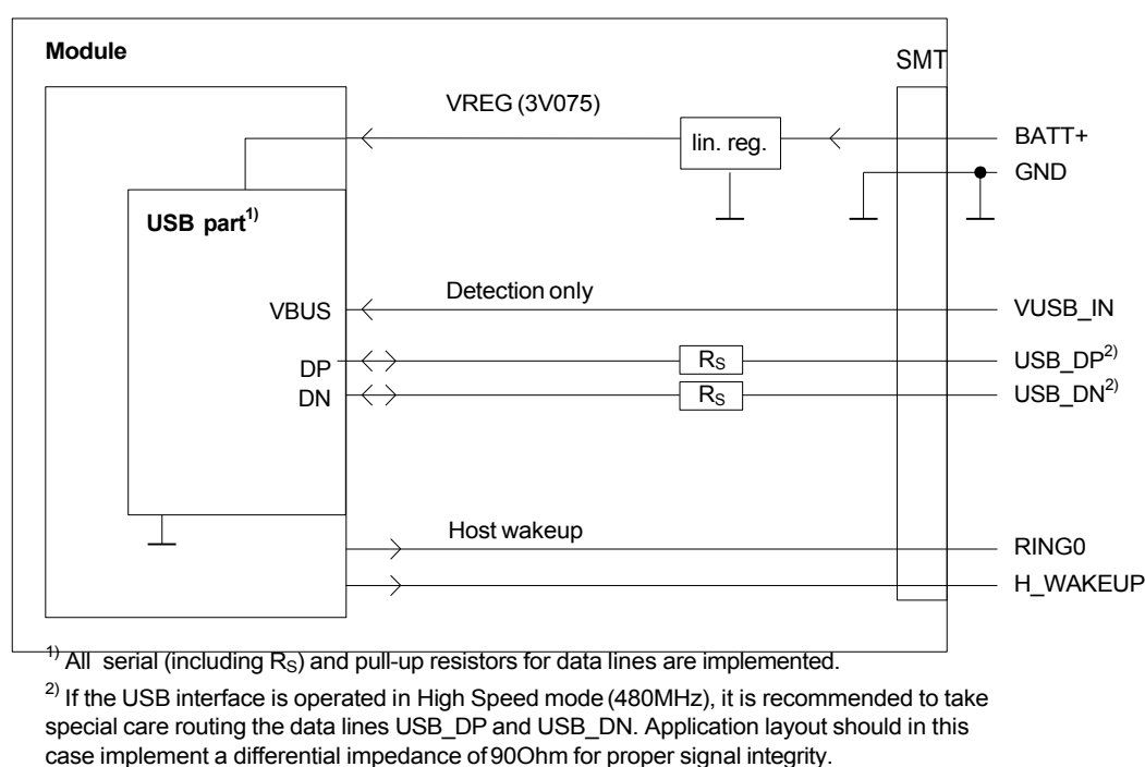
Figure 2: USB circuit
