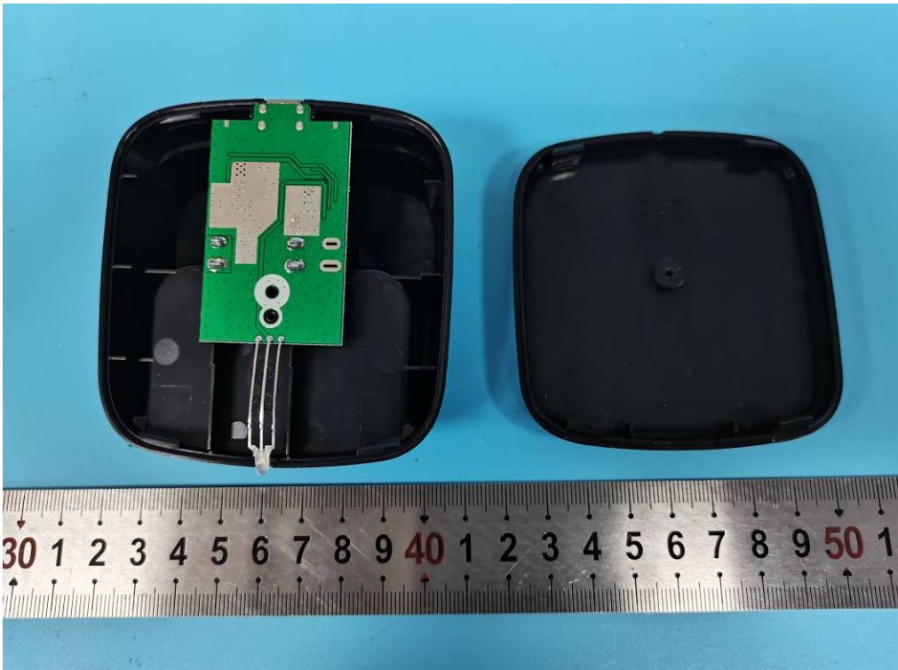
Charging base
