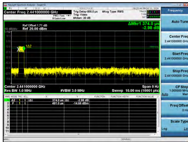
Burst(DH1)
