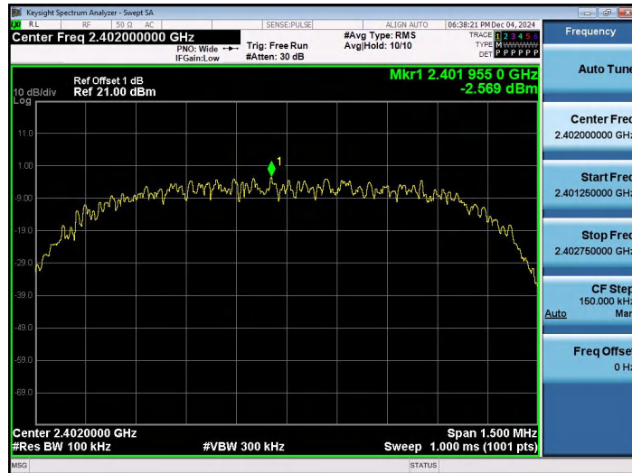
3DH5-Ant1-2402-0~Reference-PASS
