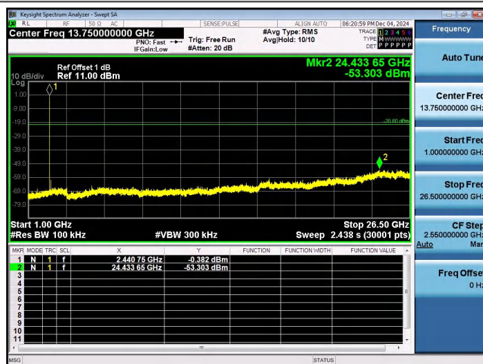
DH5-Ant1-2441-1000~26500-PASS
