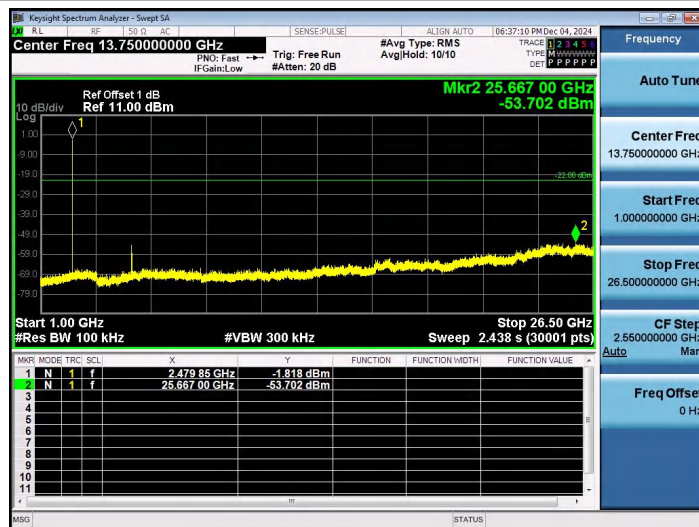
2DH5-Ant1-2480-1000~26500-PASS
