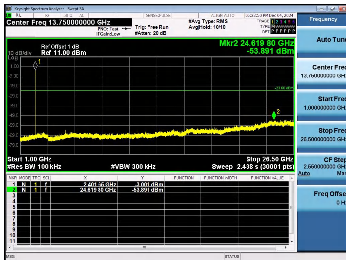
2DH5-Ant1-2402-1000~26500-PASS
