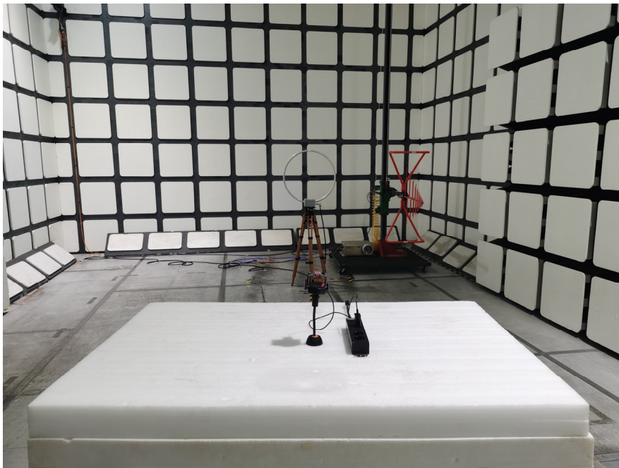
Radiated Emissions View (Below 30MHz) - Parallel
