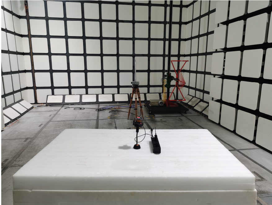
Radiated Emissions View (Below 30MHz) - Perpendicular
