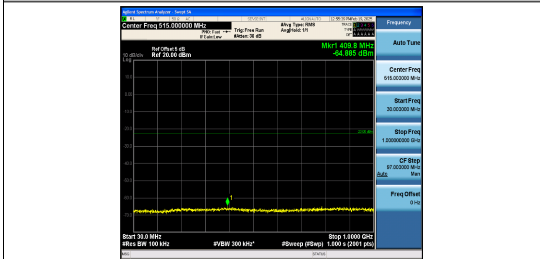
Band4_5MHz_QPSK_19975_1RB#0_30~1000_30~1000
