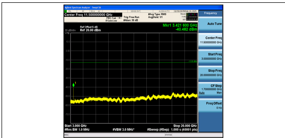
Band4_10MHz_QPSK_20000_1RB#0_3000~20000_3000~20000
