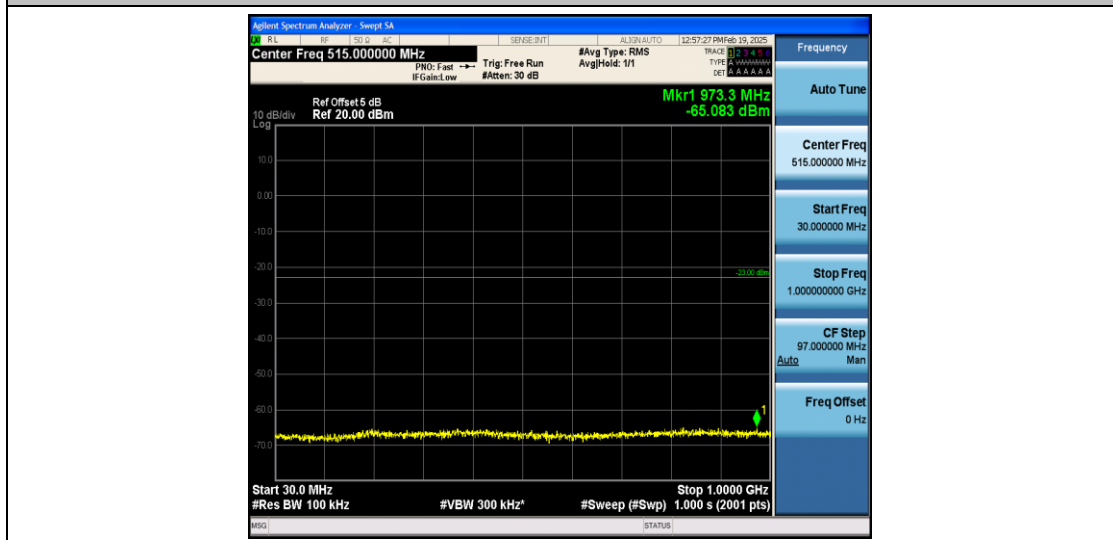
Band4_5MHz_QPSK_20175_1RB#0_30~1000_30~1000
