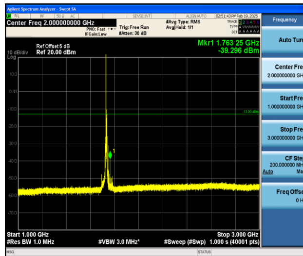
Band4_10MHz_QPSK_20175_1RB#0_1000~3000_1000~3000
