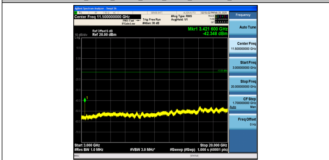
Band4_10MHz_16QAM_20000_1RB#0_3000~20000_3000~20000
