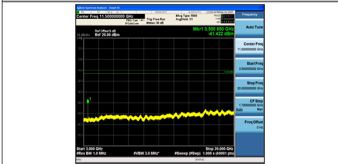
Band4_5MHz_QPSK_20375_1RB#0_3000~20000_3000~20000
