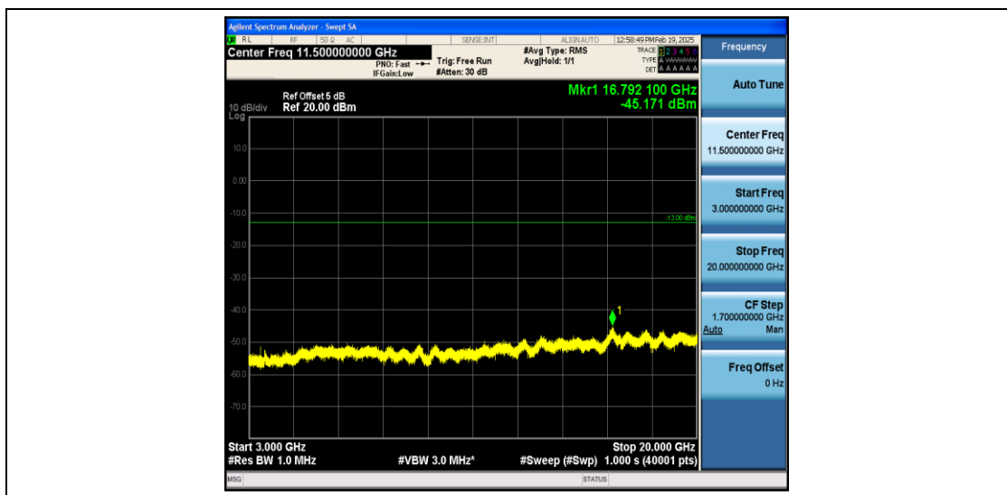
Band4_5MHz_16QAM_20175_1RB#0_3000~20000_3000~20000
