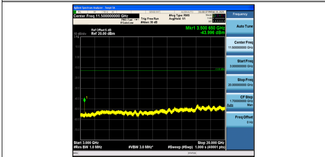
Band4_5MHz_16QAM_20375_1RB#0_3000~20000_3000~20000
