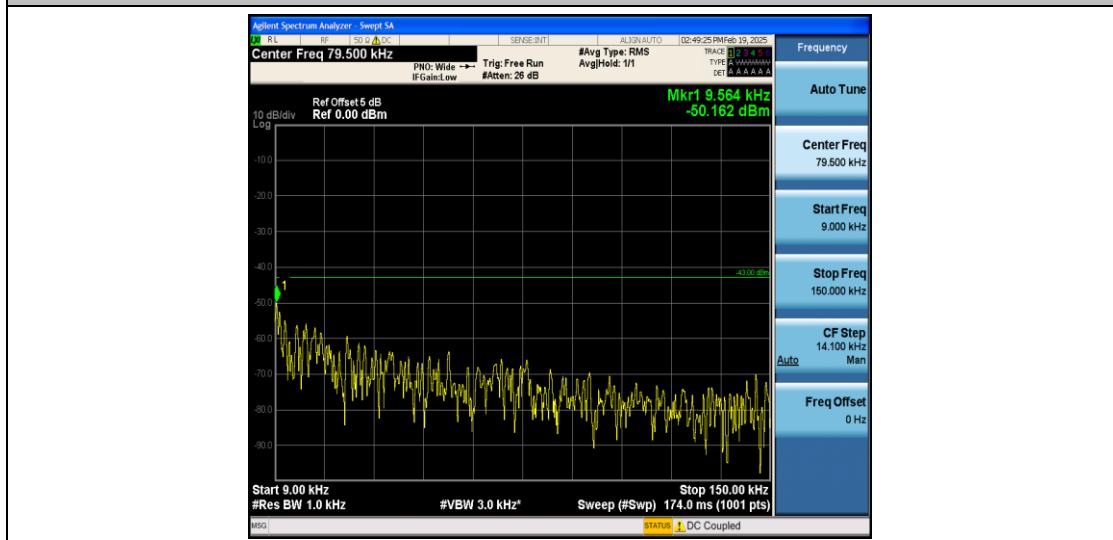
Band4_10MHz_QPSK_20000_1RB#0_0.009~0.15_0.009~0.15
