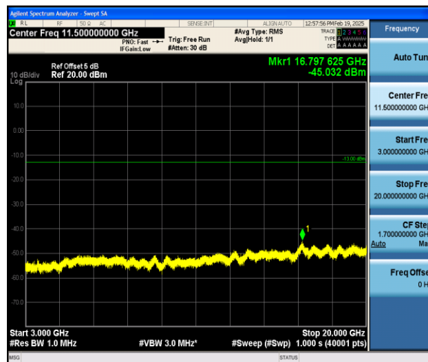
Band4_5MHz_QPSK_20175_1RB#0_3000~20000_3000~20000
