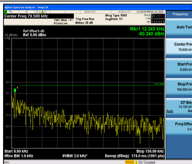
Band4_5MHz_16QAM_20175_1RB#0_0.009~0.15_0.009~0.15
