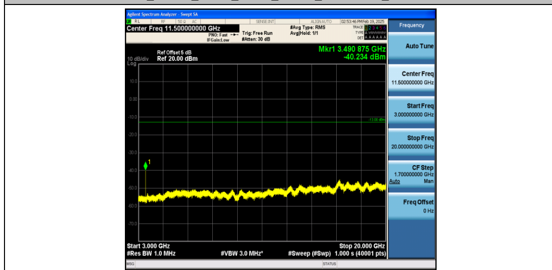
Band4_10MHz_QPSK_20350_1RB#0_3000~20000_3000~20000
