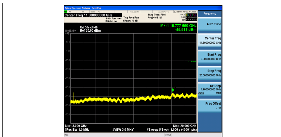
Band4_5MHz_QPSK_19975_1RB#0_3000~20000_3000~20000
