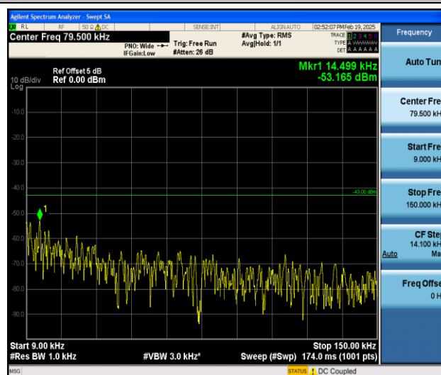
Band4_10MHz_16QAM_20175_1RB#0_0.009~0.15_0.009~0.15
