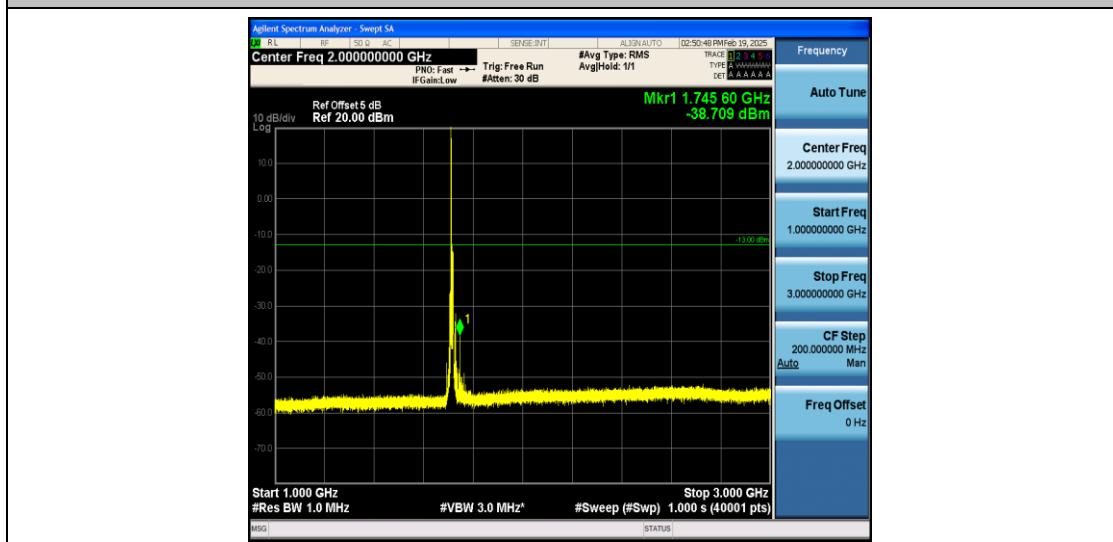
Band4_10MHz_16QAM_20000_1RB#0_1000~3000_1000~3000
