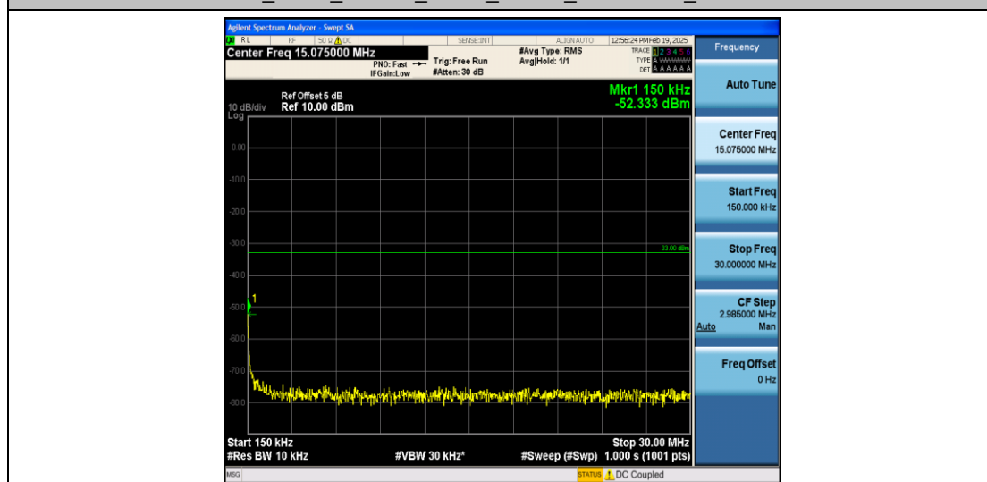
Band4_5MHz_16QAM_19975_1RB#0_0.15~30_0.15~30
