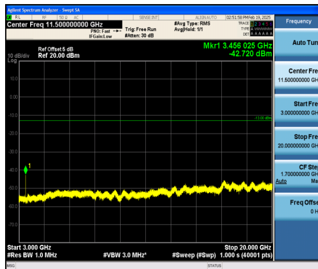
Band4_10MHz_QPSK_20175_1RB#0_3000~20000_3000~20000
