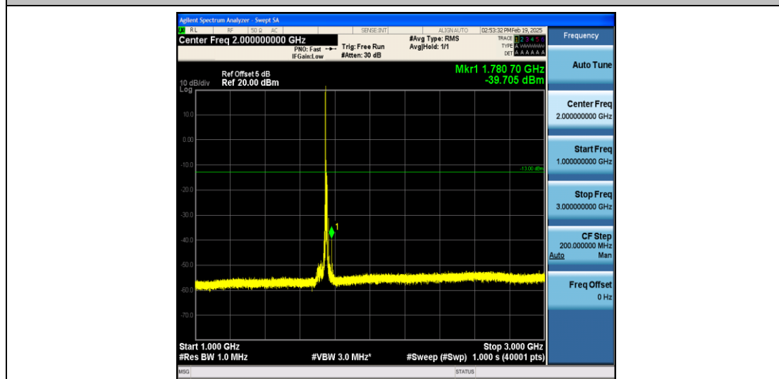
Band4_10MHz_QPSK_20350_1RB#0_1000~3000_1000~3000
