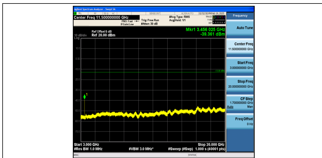
Band4_10MHz_16QAM_20175_1RB#0_3000~20000_3000~20000
