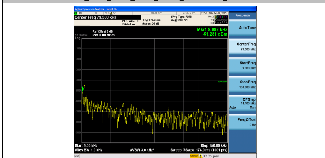
Band4_5MHz_16QAM_19975_1RB#0_0.009~0.15_0.009~0.15
