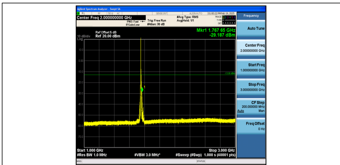
Band4_5MHz_16QAM_20375_1RB#0_1000~3000_1000~3000
