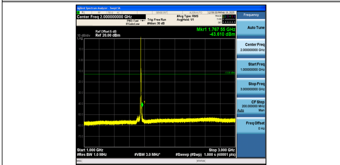
Band4_5MHz_QPSK_20375_1RB#0_1000~3000_1000~3000
