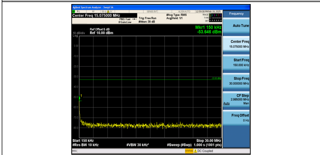
Band4_5MHz_QPSK_20375_1RB#0_0.15~30_0.15~30
