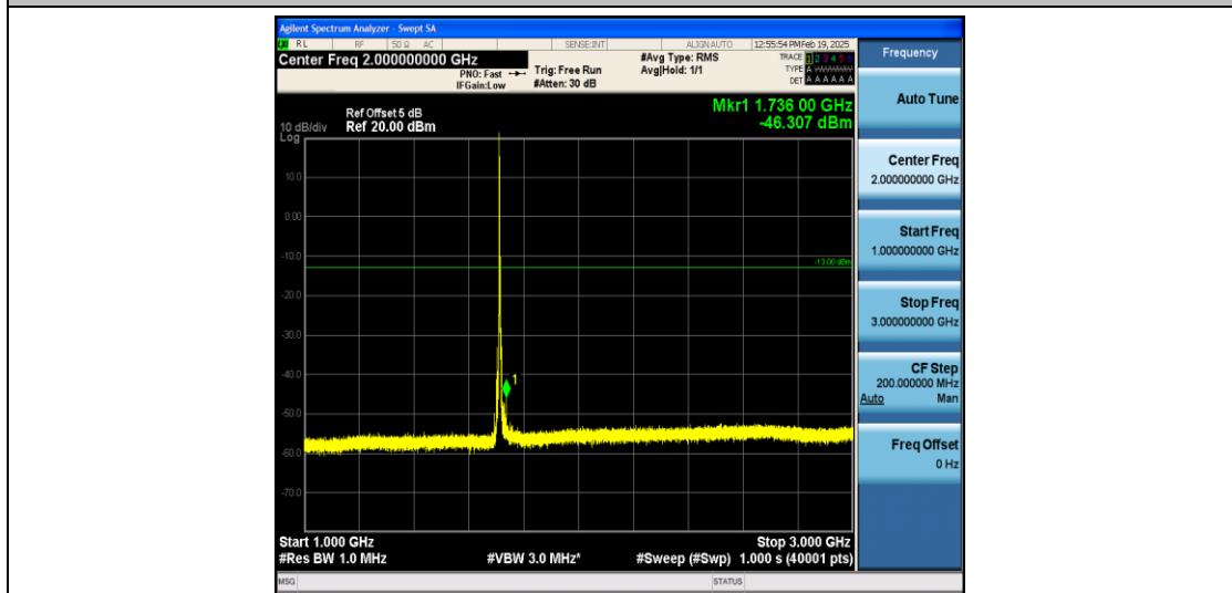
Band4_5MHz_QPSK_19975_1RB#0_1000~3000_1000~3000
