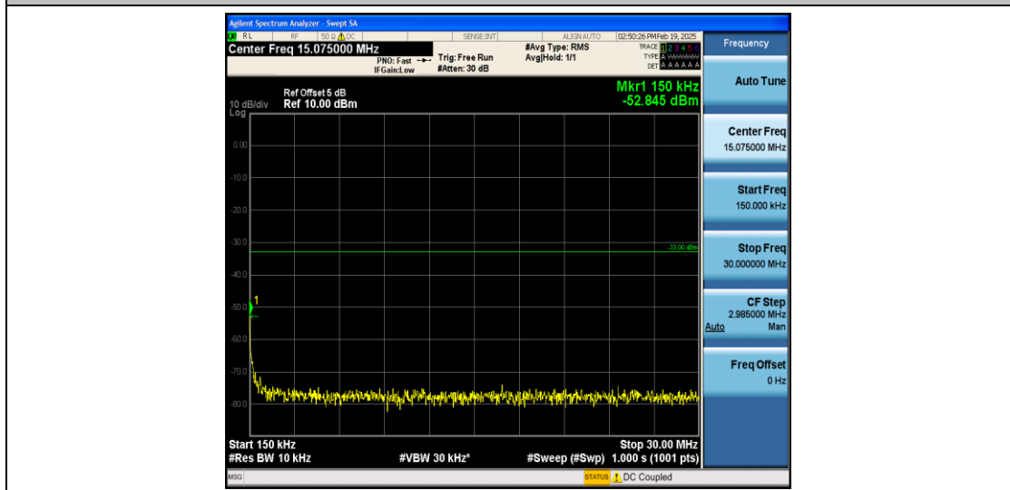
Band4_10MHz_16QAM_20000_1RB#0_0.15~30_0.15~30
