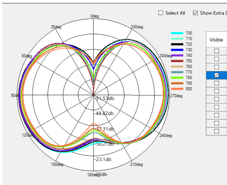
LTEB12/B17/B28 Phi=90deg
