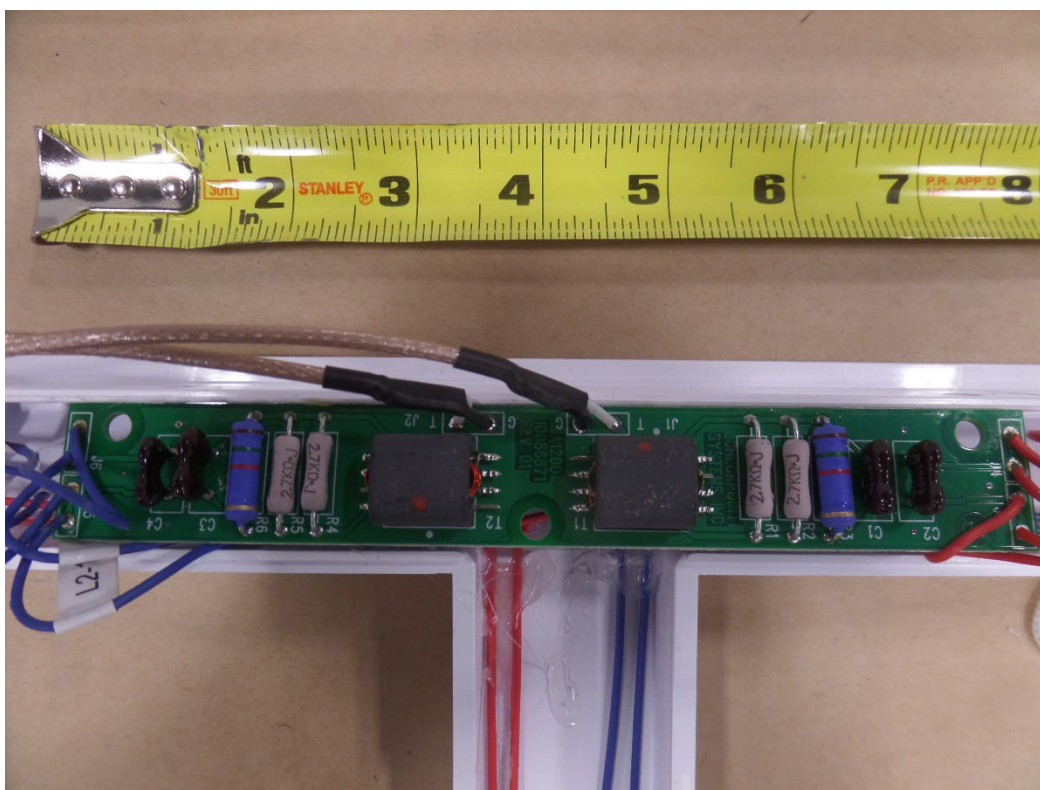
Figure 15: NP22 PRI/PAB/SAB RF ANT FRAME MATCHING BOARD TOP SIDE
