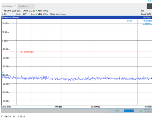
Band2-10MHz-16QAM-18650-1RB#0- Range1:30~1000MHz
