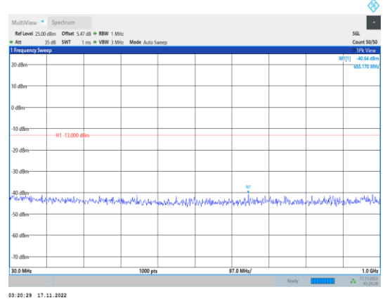
Band2-15MHz-64QAM-19125-1RB#0- Range1:30~1000MHz
