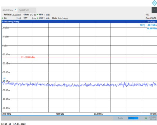
Band4-3MHz-64QAM-20175-1RB#0- Range1:30~1000MHz
