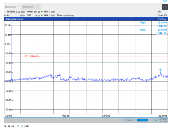
Band2-1.4MHz-16QAM-18900-1RB#0- Range2:1000~20000MHz
