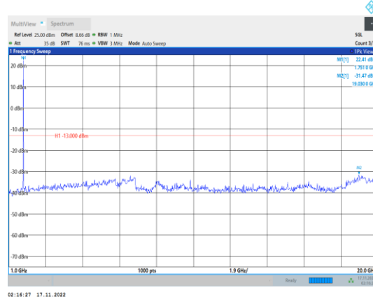
Band4-3MHz-64QAM-20385-1RB#0- Range2:1000~20000MHz
