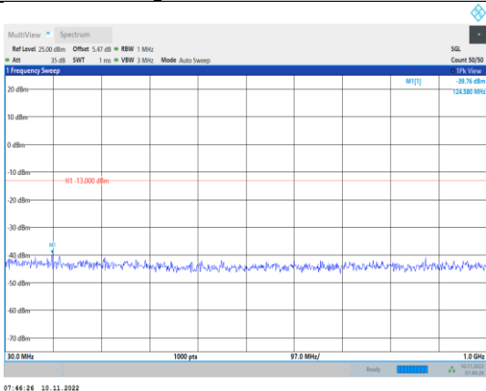
Band4-3MHz-16QAM-20175-1RB#0- Range1:30~1000MHz
