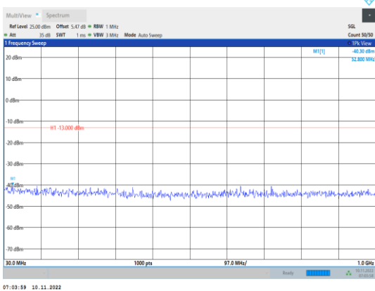
Band2-10MHz-QPSK-18650-1RB#0- Range1:30~1000MHz
