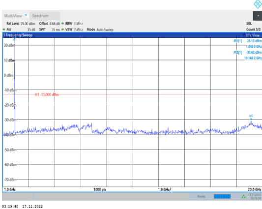
Band2-15MHz-64QAM-18675-1RB#0- Range2:1000~20000MHz
