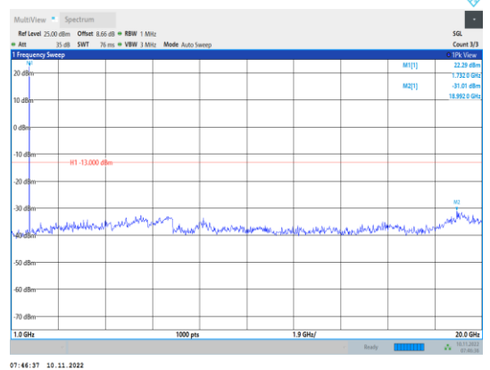
Band4-3MHz-16QAM-20175-1RB#0- Range2:1000~20000MHz
