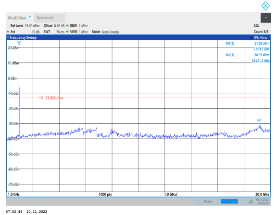
Band2-1.4MHz-16QAM-19193-1RB#0- Range2:1000~20000MHz
