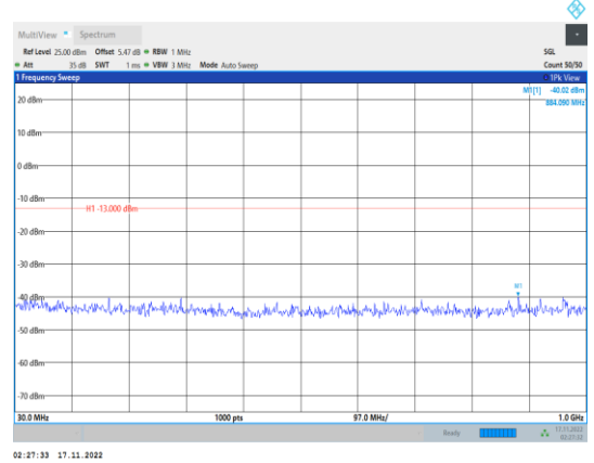
Band4-1.4MHz-64QAM-20393-1RB#0- Range1:30~1000MHz
