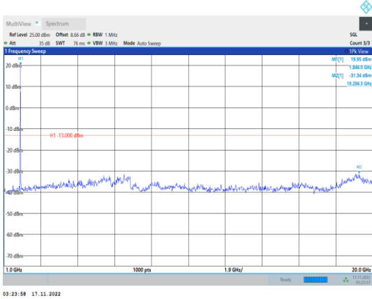
Band2-5MHz-64QAM-18625-1RB#0- Range2:1000~20000MHz
