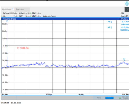
Band2-10MHz-16QAM-18650-1RB#0- Range2:1000~20000MHz
