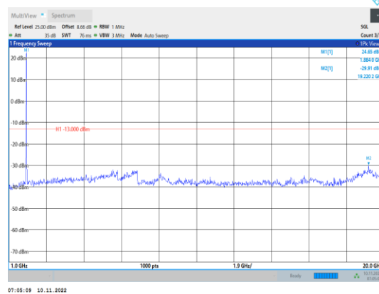
Band2-10MHz-QPSK-18900-1RB#0- Range2:1000~20000MHz
