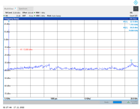
Band4-1.4MHz-64QAM-20393-1RB#0- Range2:1000~20000MHz
