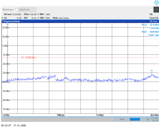
Band4-3MHz-64QAM-19965-1RB#0- Range2:1000~20000MHz
