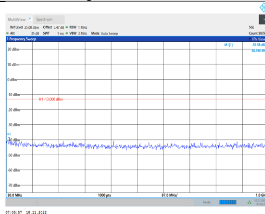
Band2-10MHz-QPSK-19150-1RB#0- Range1:30~1000MHz
