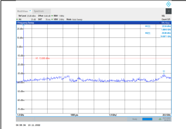
Band2-1.4MHz-QPSK-18900-1RB#0-Range2:1000~20000MHz
