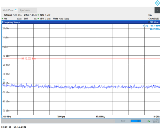
Band2-15MHz-64QAM-18900-1RB#0- Range1:30~1000MHz
