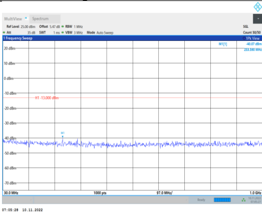
Band2-10MHz-16QAM-18900-1RB#0- Range1:30~1000MHz
