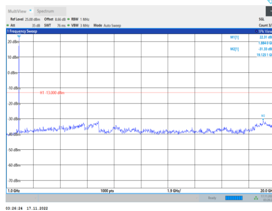
Band2-3MHz-64QAM-18900-1RB#0- Range2:1000~20000MHz
