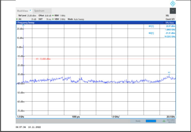
Band2-1.4MHz-QPSK-18607-1RB#0-Range2:1000~20000MHz
