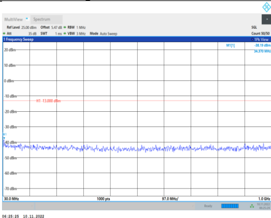
Band4-1.4MHz-QPSK-20175-1RB#0- Range1:30~1000MHz
