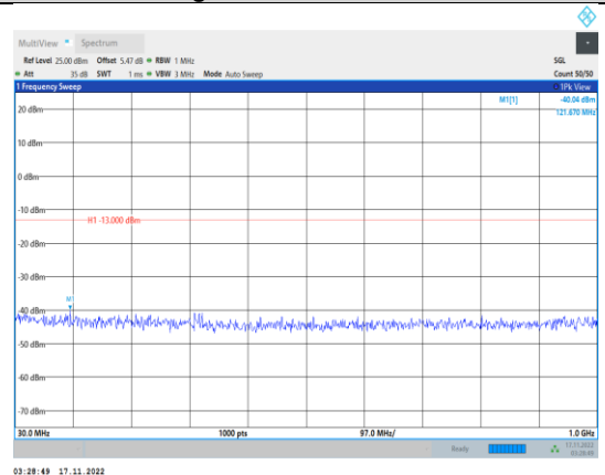
Band2-1.4MHz-64QAM-19193-1RB#0- Range1:30~1000MHz
