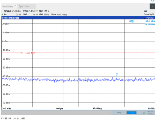
Band2-15MHz-16QAM-18675-1RB#0- Range1:30~1000MHz
