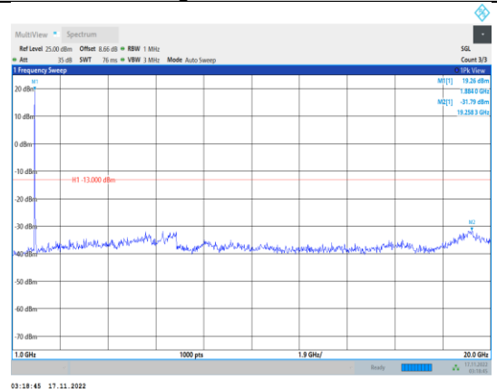
Band2-20MHz-64QAM-19100-1RB#0- Range2:1000~20000MHz
