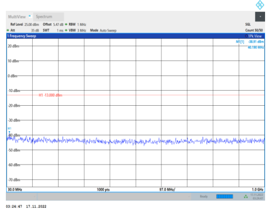
Band2-5MHz-64QAM-19175-1RB#0- Range1:30~1000MHz
