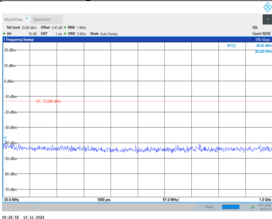
Band4-1.4MHz-16QAM-20393-1RB#0- Range1:30~1000MHz
