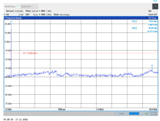
Band2-1.4MHz-64QAM-18900-1RB#0- Range2:1000~20000MHz
