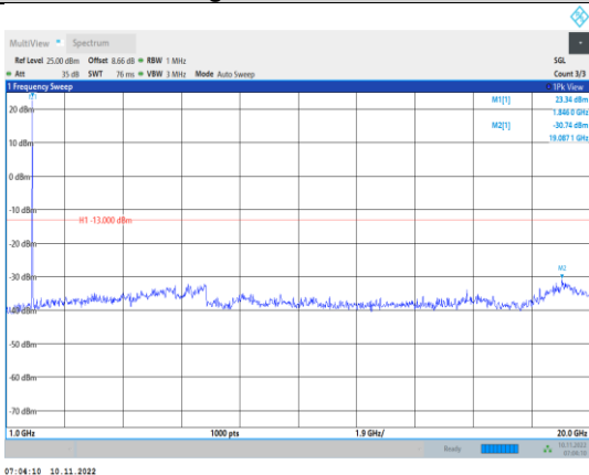
Band2-10MHz-QPSK-18650-1RB#0- Range2:1000~20000MHz
