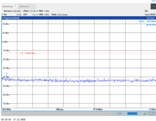
Band4-3MHz-64QAM-19965-1RB#0- Range1:30~1000MHz
