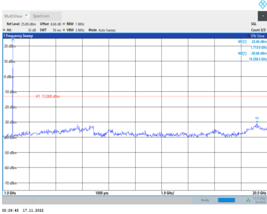
Band4-1.4MHz-64QAM-19957-1RB#0- Range2:1000~20000MHz
