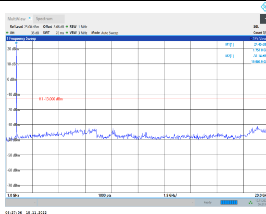
Band4-1.4MHz-16QAM-20393-1RB#0- Range2:1000~20000MHz
