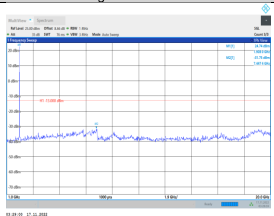
Band2-1.4MHz-64QAM-19193-1RB#0- Range2:1000~20000MHz
