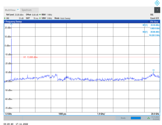
Band2-15MHz-64QAM-19125-1RB#0- Range2:1000~20000MHz
