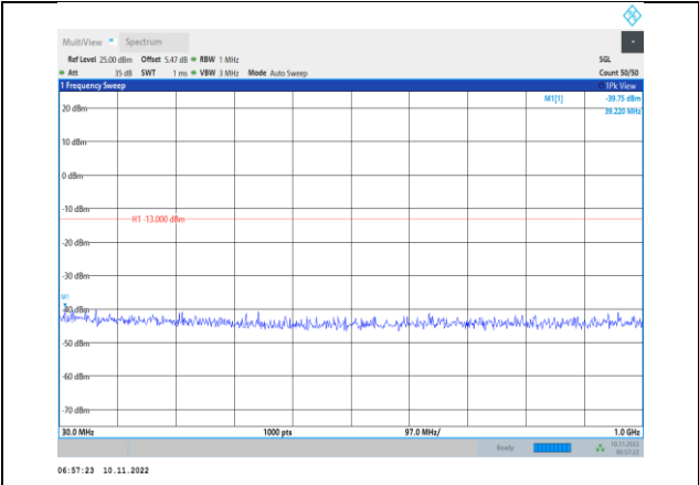
Band2-1.4MHz-QPSK-18607-1RB#0-Range1:30~1000MHz
