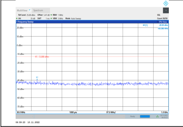
Band2-1.4MHz-QPSK-19193-1RB#0-Range1:30~1000MHz
