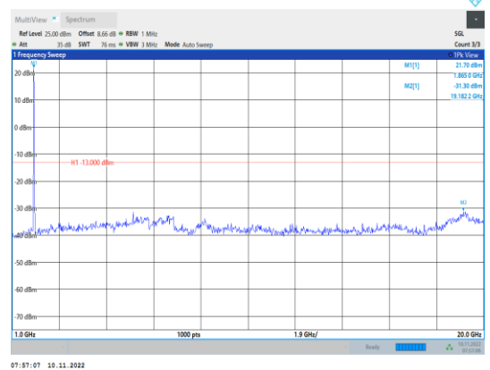
Band2-15MHz-16QAM-18900-1RB#0- Range2:1000~20000MHz
