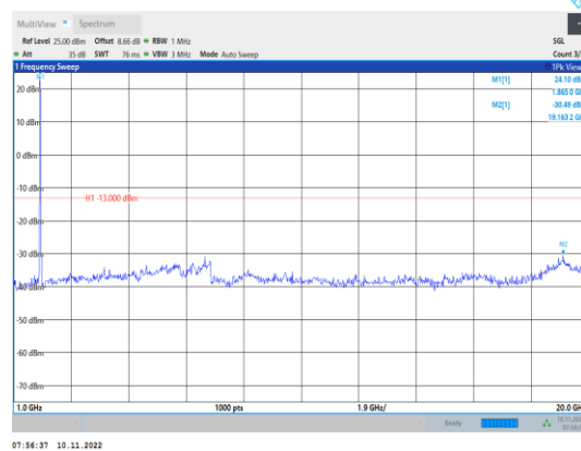
Band2-15MHz-QPSK-18900-1RB#0- Range2:1000~20000MHz
