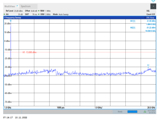
Band2-3MHz-16QAM-18900-1RB#0- Range2:1000~20000MHz
