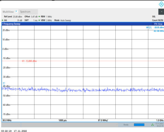
Band2-10MHz-64QAM-18900-1RB#0- Range1:30~1000MHz
