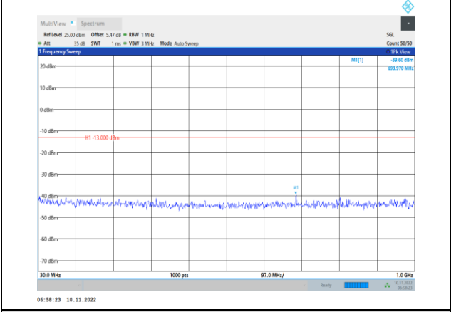
Band2-1.4MHz-QPSK-18900-1RB#0-Range1:30~1000MHz
