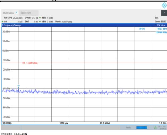
Band2-10MHz-QPSK-18900-1RB#0- Range1:30~1000MHz
