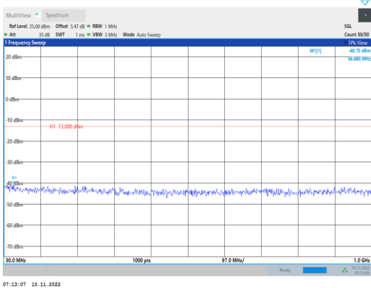
Band2-3MHz-16QAM-18615-1RB#0- Range1:30~1000MHz
