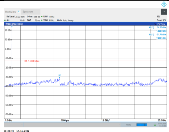
Band2-10MHz-64QAM-19150-1RB#0- Range2:1000~20000MHz
