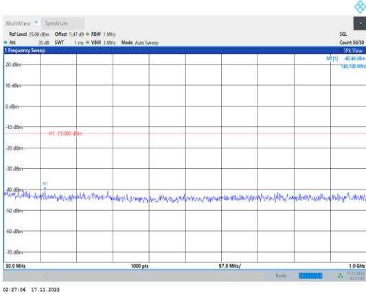
Band4-1.4MHz-64QAM-20175-1RB#0- Range1:30~1000MHz
