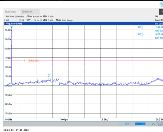
Band2-3MHz-64QAM-19185-1RB#0- Range2:1000~20000MHz
