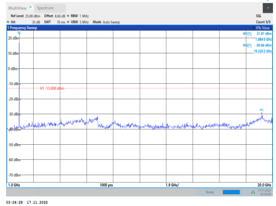
Band2-5MHz-64QAM-18900-1RB#0- Range2:1000~20000MHz
