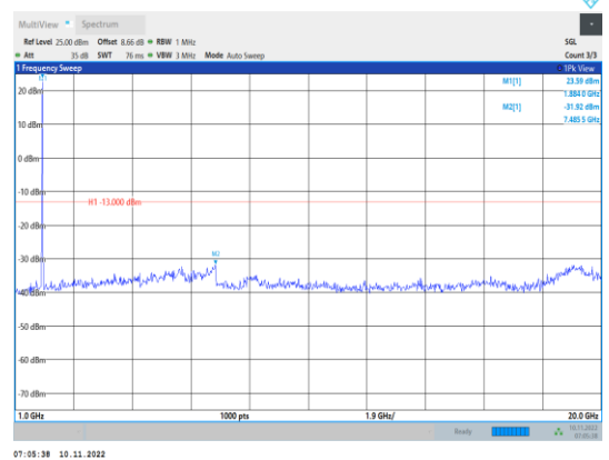
Band2-10MHz-16QAM-18900-1RB#0- Range2:1000~20000MHz
