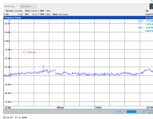
Band4-3MHz-64QAM-20175-1RB#0- Range2:1000~20000MHz
