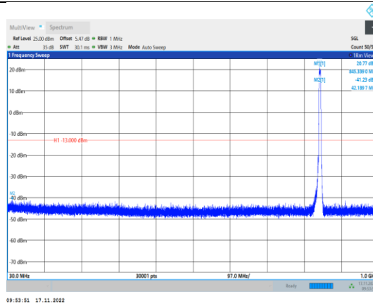
Band5-4233-30~1000MHz
