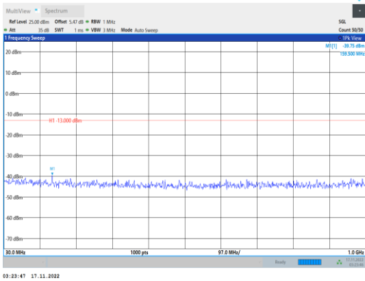
Band2-5MHz-64QAM-18625-1RB#0- Range1:30~1000MHz
