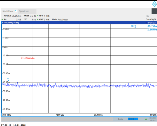
Band2-15MHz-QPSK-18900-1RB#0- Range1:30~1000MHz
