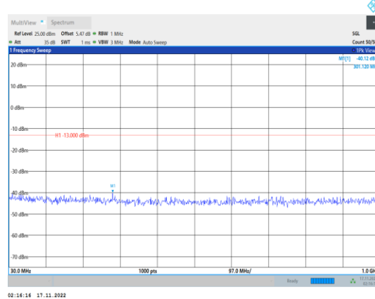
Band4-3MHz-64QAM-20385-1RB#0- Range1:30~1000MHz
