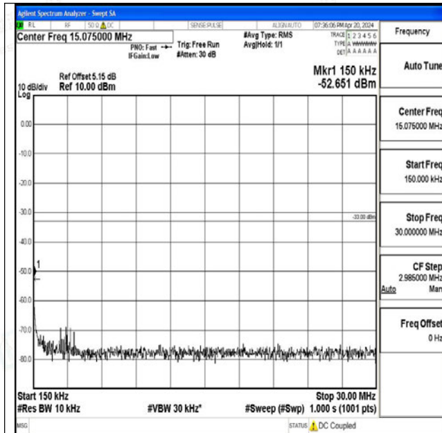
Band66_3MHz_16QAM_131987_1RB#0_0.15~30_0.15~30
