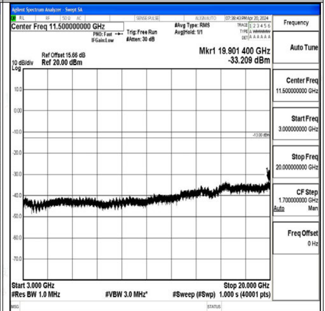
Band66_3MHz_16QAM_132657_1RB#0_3000~20000_3000~20000
