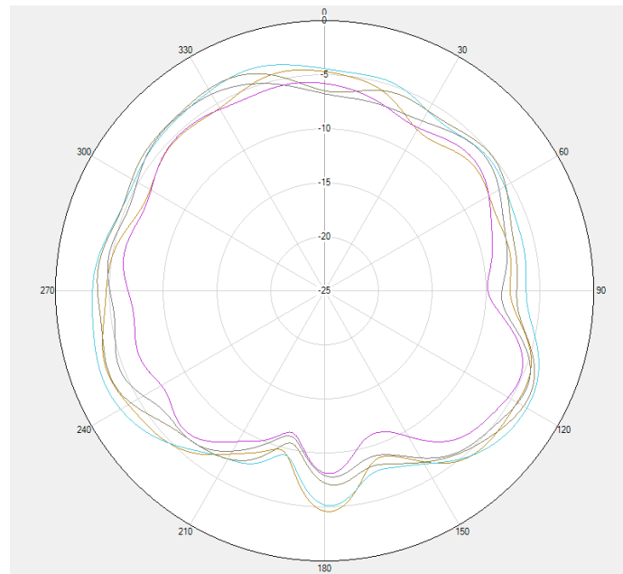
GSM900,B8,N8,WB8 \Phi=90^\circ
