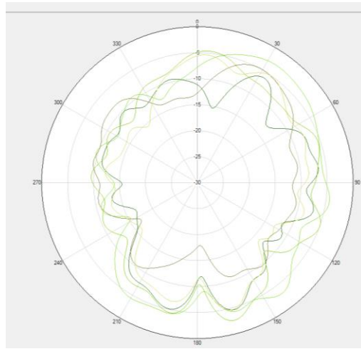
B42/NR n77/78 \Phi=90\text{deg}
