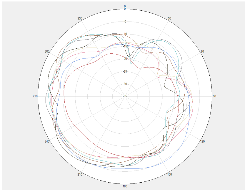
B42/N77/78&wifi 5G \Phi=0^\circ
