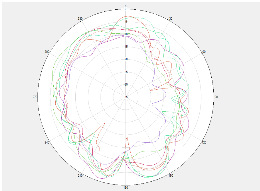
B42/N77/78&wifi 5G \Phi=90^\circ
