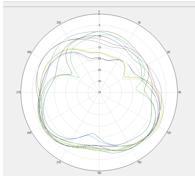
B1/B3/B7/B38/B40/B41 \Phi = 0^\circ
