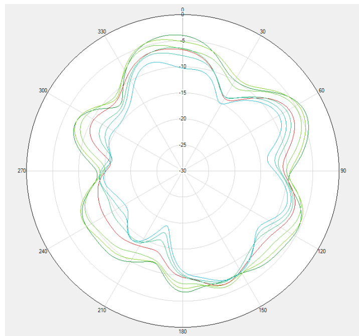
GSM900,B8,N8,WB8 \Theta=90^\circ
