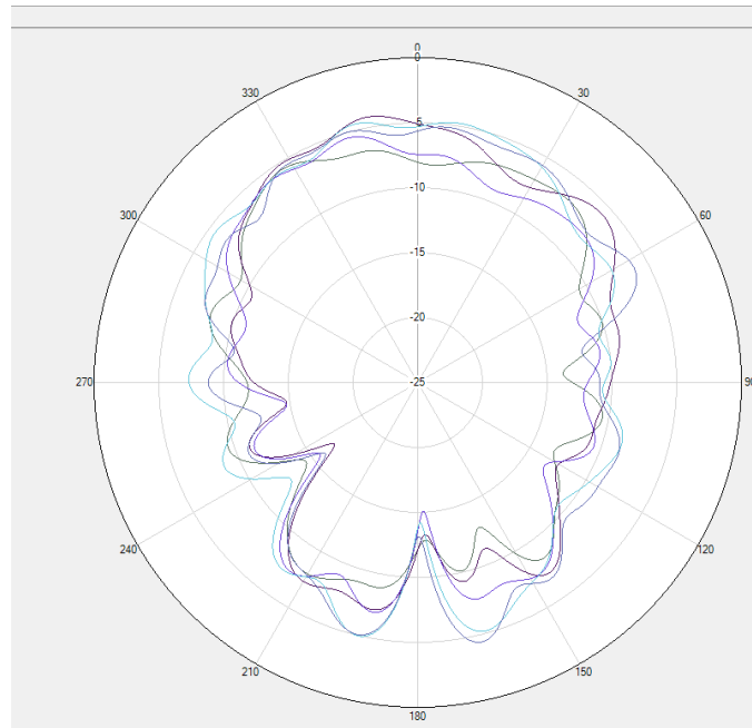
B42/N77/N78 Phi=90deg
