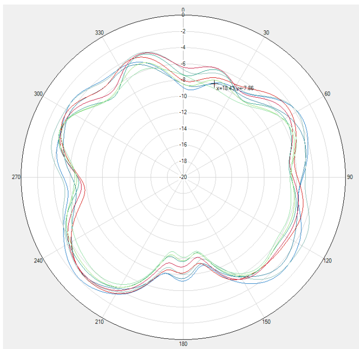
GSM900,B8,N8,WB8 \Phi=90^\circ
