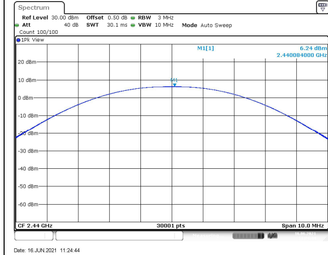
Channel 19 (2440MHz)
