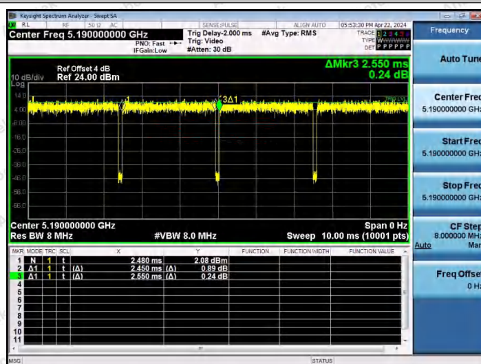
NTNV-11AX40MIMO-Ant2-5190
