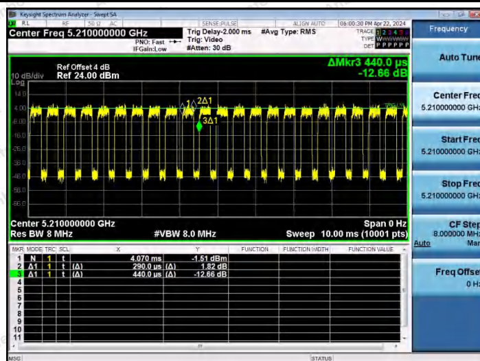
NTNV-11AX80MIMO-Ant2-5210
