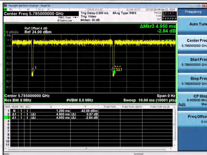
NTNV-11AX20MIMO-Ant2-5785
