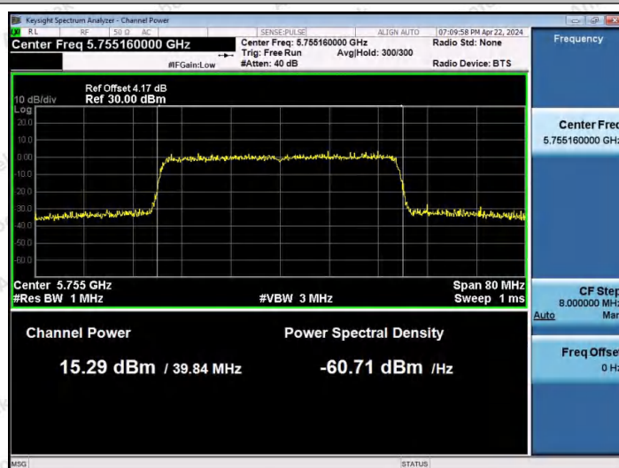
11AX40MIMO-Ant2-5755-PASS
