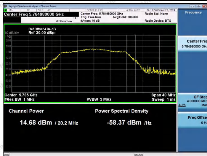
11A-Ant2-5785-PASS
