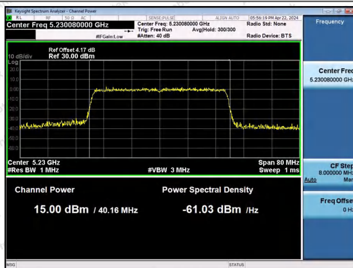
11AX40MIMO-Ant2-5230-PASS
