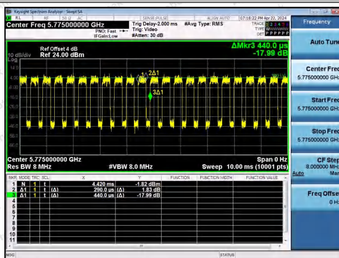
NTNV-11AX80MIMO-Ant2-5775
