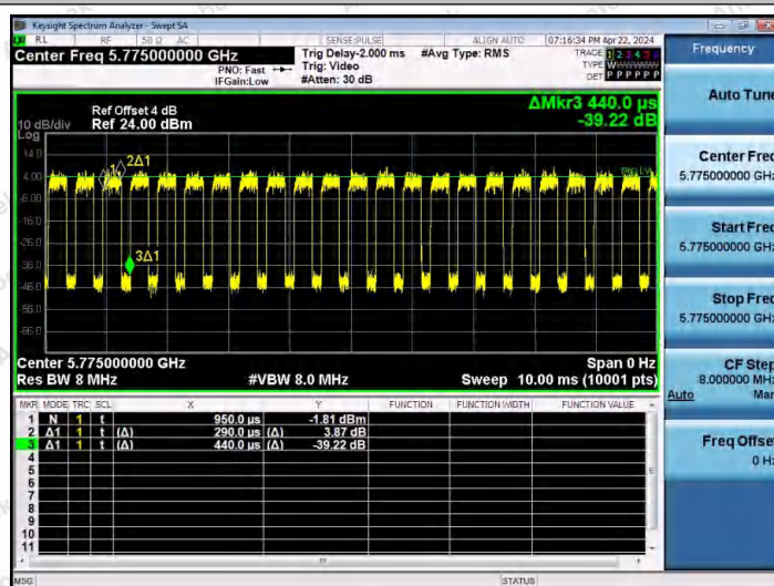
NTNV-11AX80MIMO-Ant1-5775
