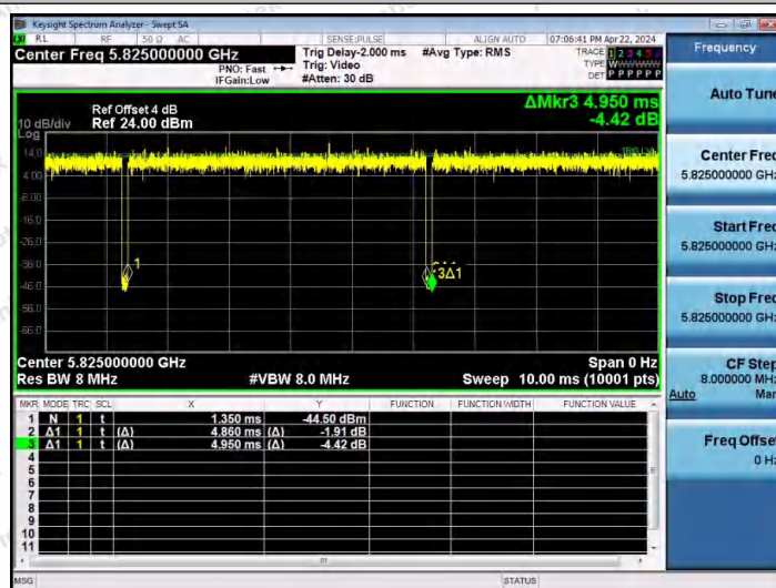
NTNV-11AX20MIMO-Ant2-5825
