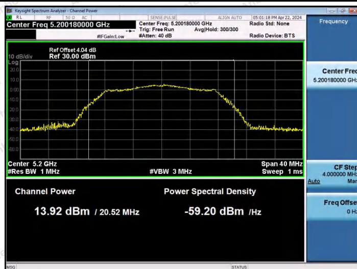
11A-Ant2-5200-PASS
