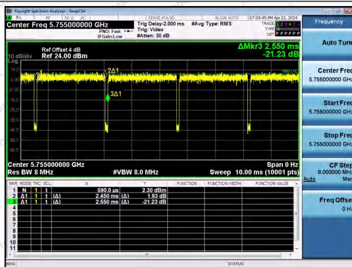
NTNV-11AX40MIMO-Ant2-5755
