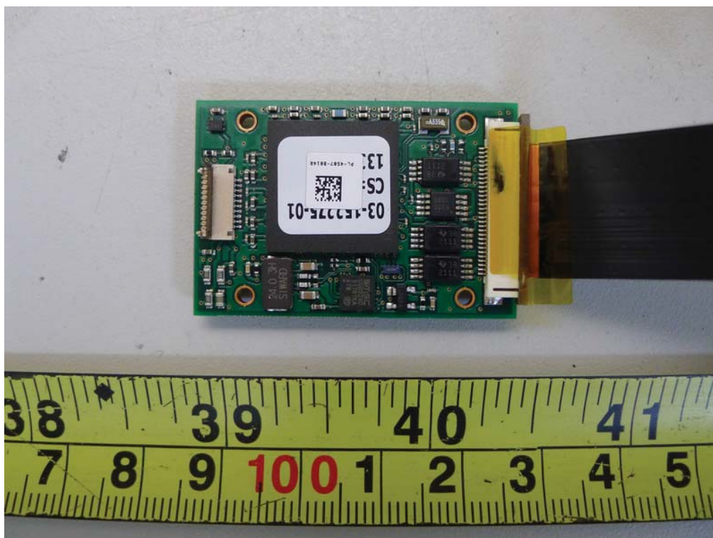
Reader: SE-4500+PL4507
