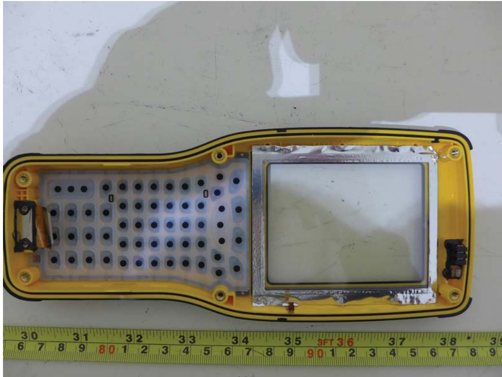
Keypad: 53 Keys
