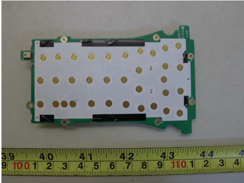
Keypad: 30 Keys
