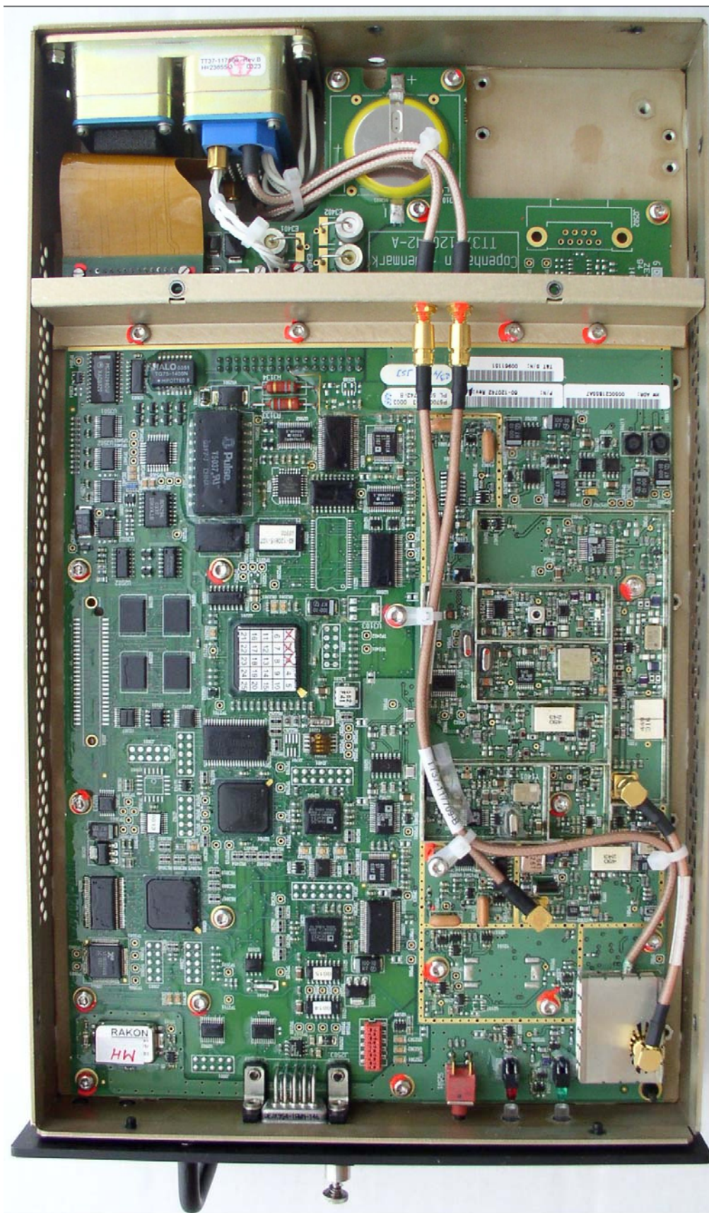
TT93-120742 – Top Side
