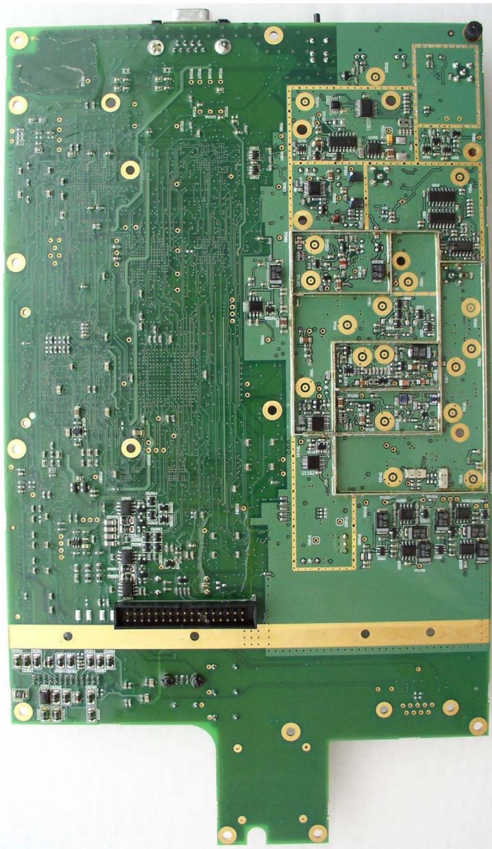
TT93-120742 – Bottom Side
