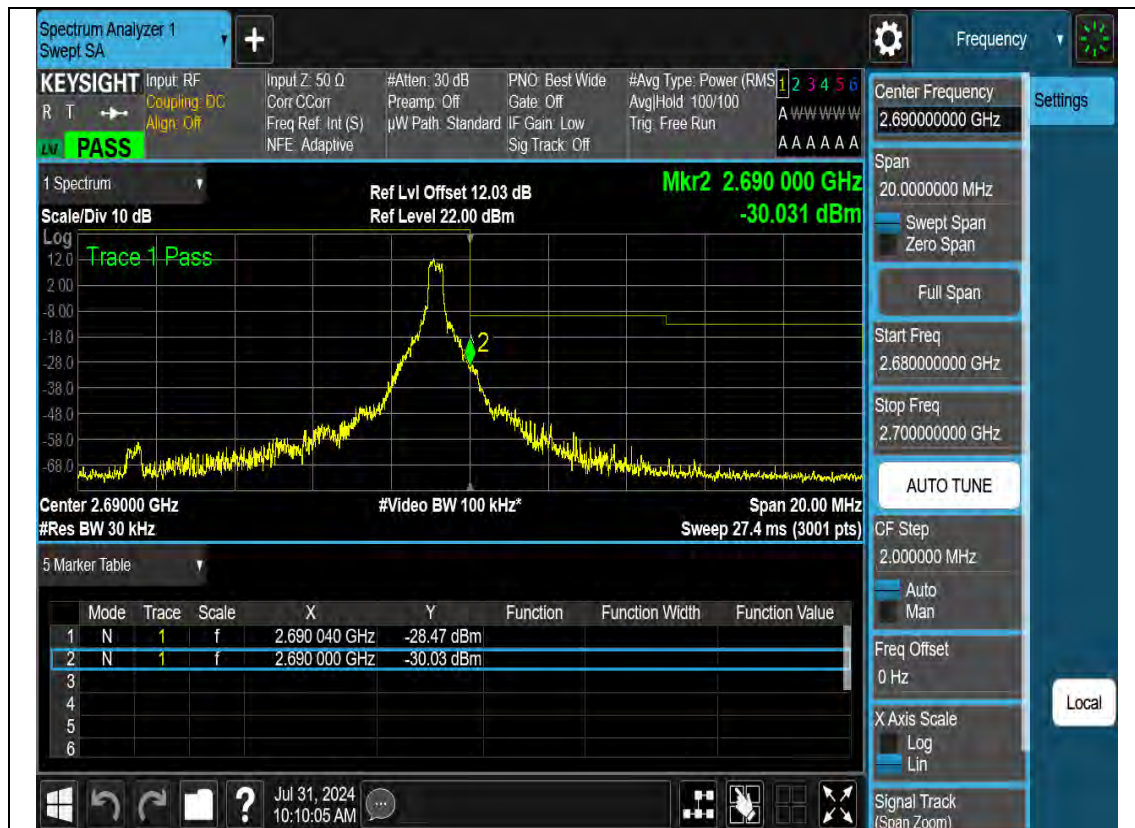
N41-10M-Bandedge-H-CP-OFDM-QPSK-Outer Full
