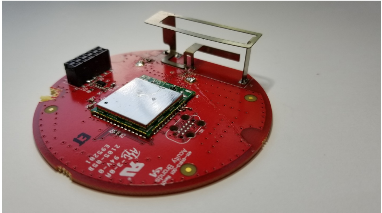
New Stamped Antenna with PCB.
