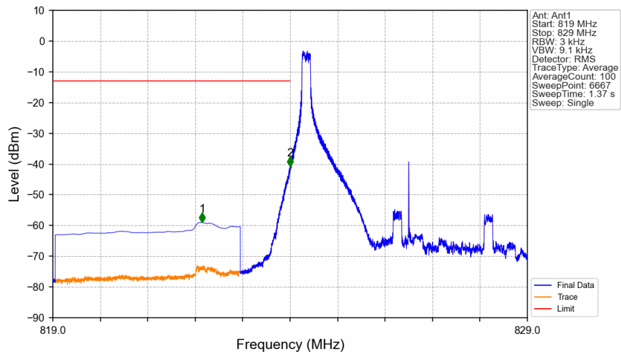
Band26b_5MHz_QPSK_LCH_826.5MHz_RB_1_0_NTNV
