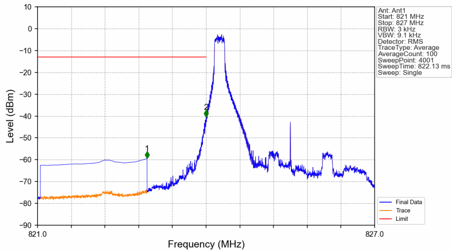
Band26b_3MHz_QPSK_LCH_825.5MHz_RB_1_0_NTNV
