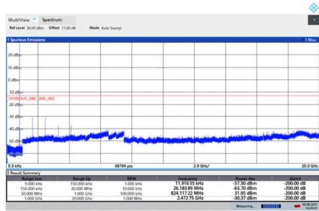
GPRS 850 CH-Middle 9kHz ~ 20GHz
