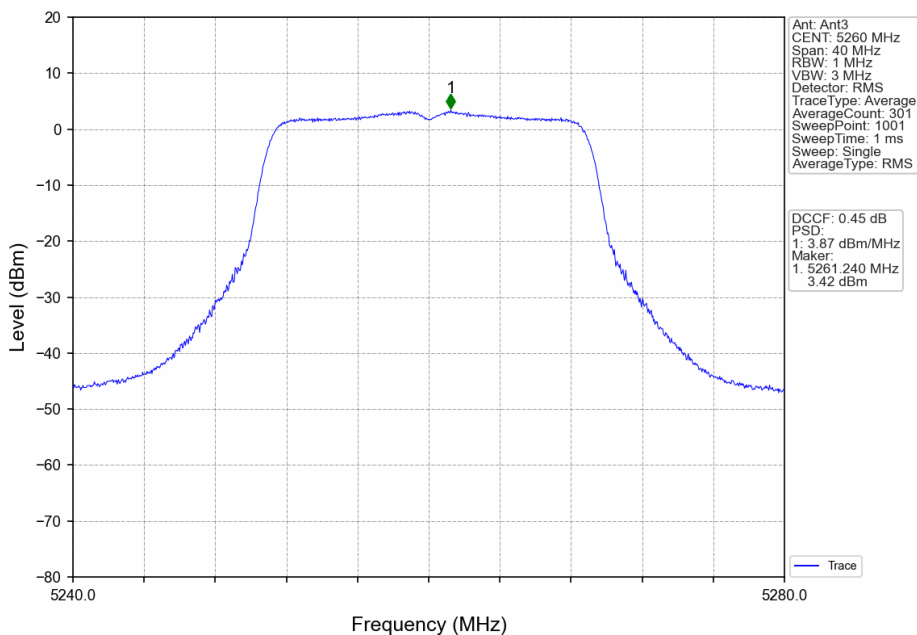
802.11ac(VHT20)_LCH_5260MHz_Ant3_NTNV
