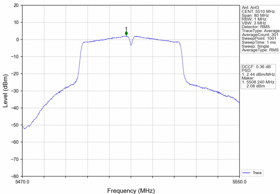
802.11n(HT40)_LCH_5510MHz_Ant3_NTNV
