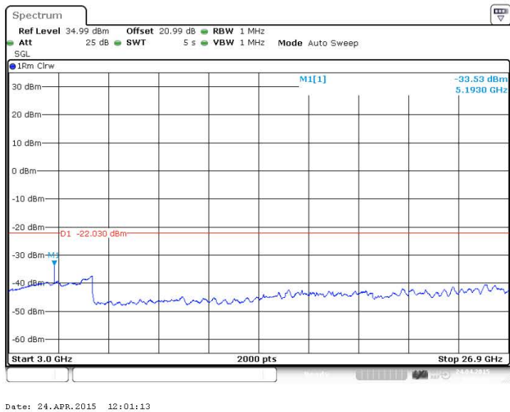
Figure 106 Spurious Emissions (3GHz – 26.900GHz) – 64QAM (2593.0 MHz) (10MHz Channel BW)
