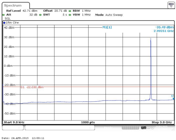
Figure 105 Spurious Emissions (9kHz – 3GHz) – 64QAM (2593.0 MHz) (10MHz Channel BW)
