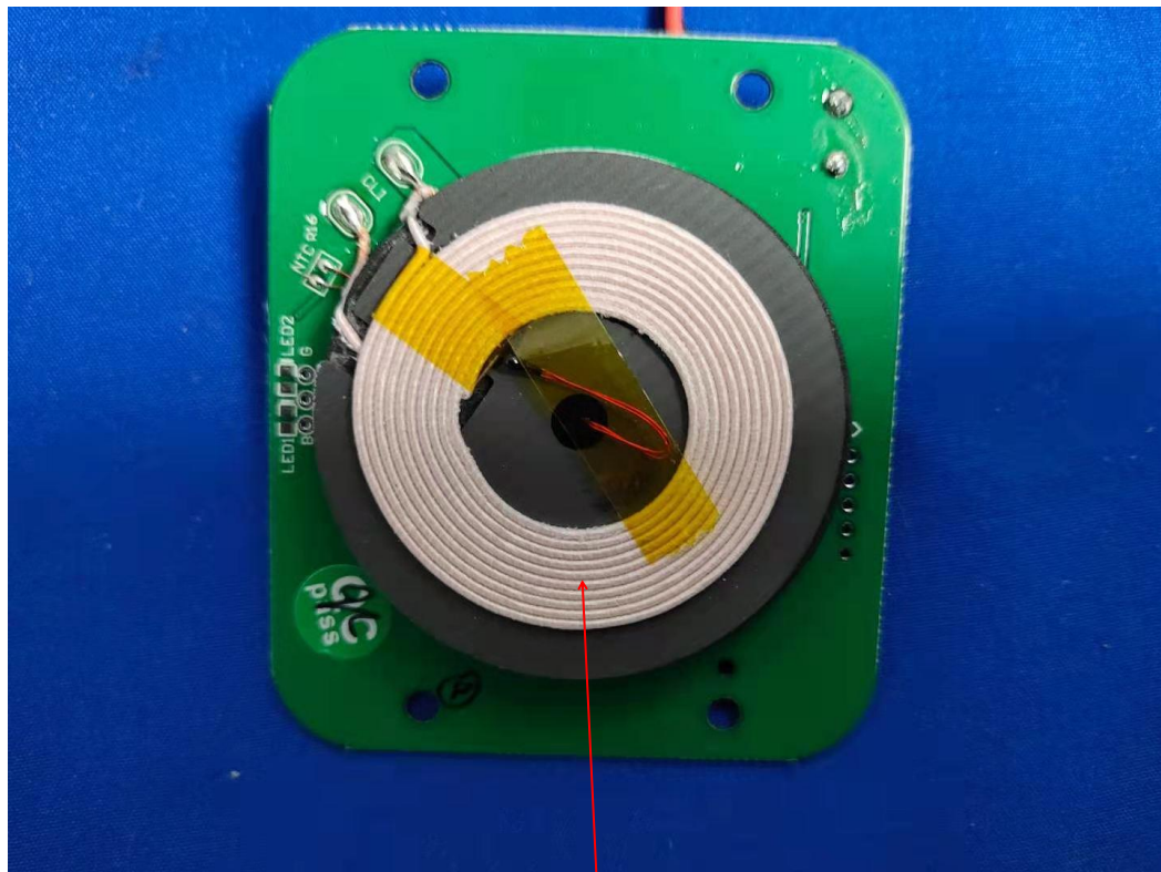
Coil ANT
