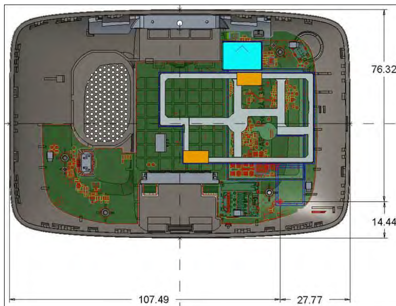
Fig.11 antenna location
