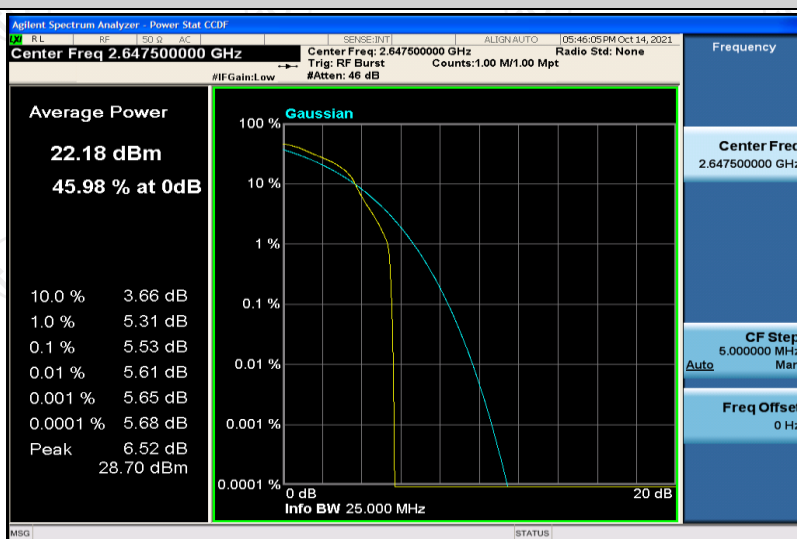
Band41-15MHz-16QAM-41165-75RB#0
