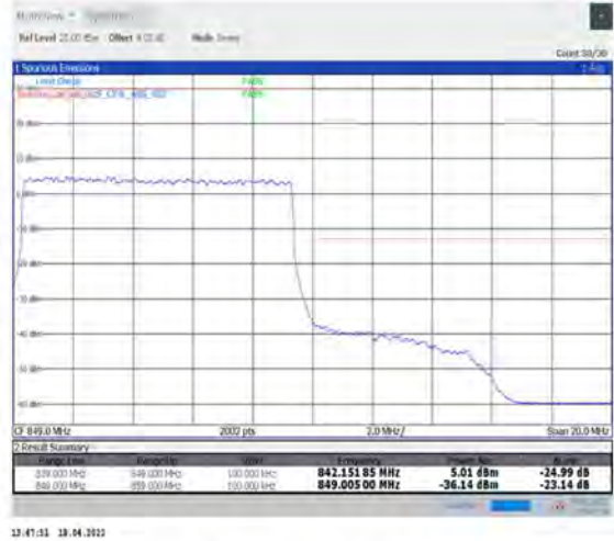
1-N5--15-10-H-3-DFT-PI2BPSK-Outer_Full-50@0-Ant1-seegraph-PASS-see graph
