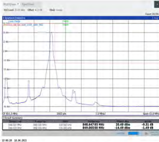
1-N5--15-5-H-2-DFT-PI2BPSK-Edge_1RB_Right-1@24-Ant1-seegraph-PASS-see graph
