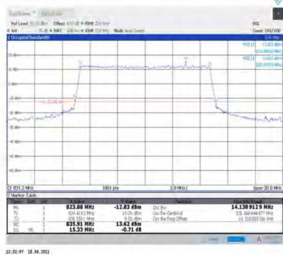
1-N5--15-15-L-6-CP-QPSK-Outer_Full-79@0-Ant1-14.139-15.330-≤15-PASS
