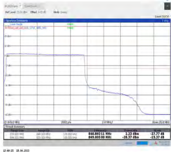
1-N5--15-10-H-6-CP-QPSK-Outer_Full-52@0-Ant1-seegraph-PASS-see graph
