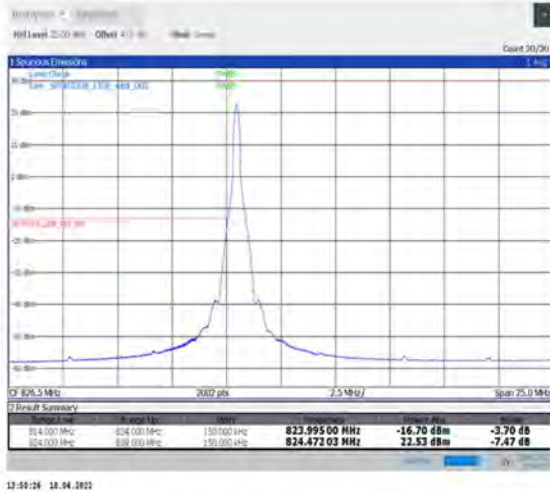
1-N5--15-15-L-1-DFT-PI2BPSK-Edge_1RB_Left-1@0-Ant1-seegraph-PASS-see graph
