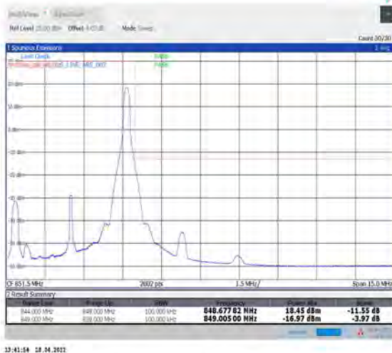
1-N5--15-5-H-5-CP-QPSK-Edge_1RB_Right-1@24-Ant1-seegraph-PASS-see graph
