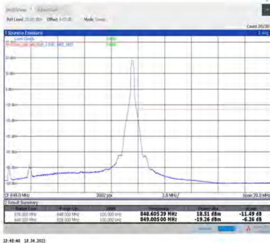
1-N5--15-10-H-5-CP-QPSK-Edge_1RB_Right-1@51-Ant1-seegraph-PASS-see graph
