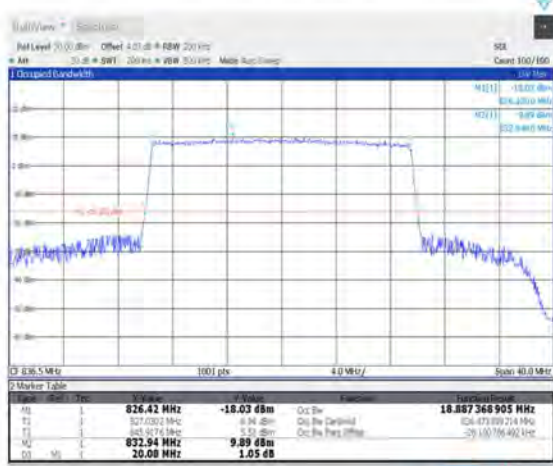
1-N5--15-20-M-9-CP-256QAM-Outer_Full-106@0- Ant1-18.887-20.080-≤20-PASS
