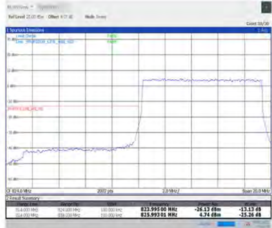
1-N5--15-10-L-3-DFT-PI2BPSK-Outer_Full-50@0-Ant1-seegraph-PASS-see graph
