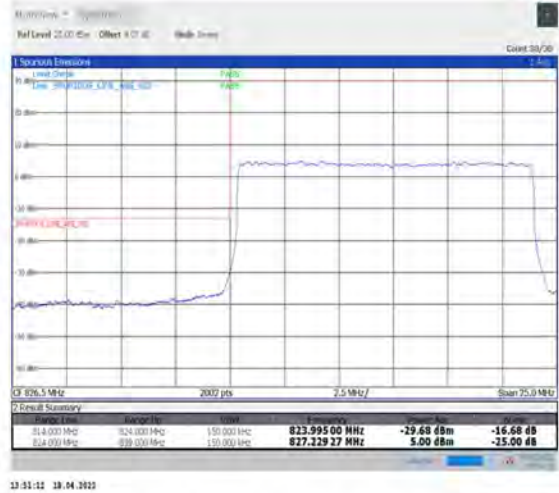
1-N5--15-15-L-3-DFT-PI2BPSK-Outer_Full-75@0-Ant1-seegraph-PASS-see graph
