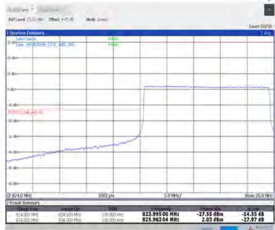
1-N5--15-10-L-6-CP-QPSK-Outer_Full-52@0-Ant1-seegraph-PASS-see graph
