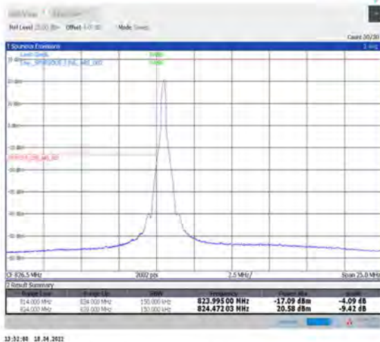
1-N5--15-15-L-4-CP-QPSK-Edge_1RB_Left-1@0-Ant1-seegraph-PASS-see graph
