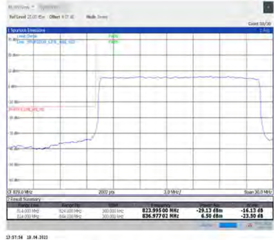
1-N5--15-20-L-3-DFT-PI2BPSK-Outer_Full-100@0-Ant1-seegraph-PASS-see graph
