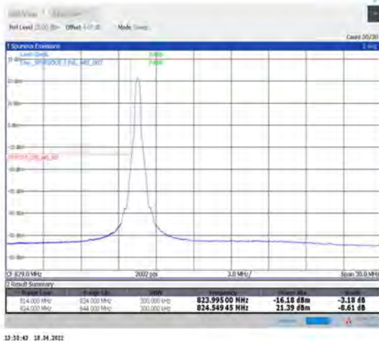
1-N5--15-20-L-4-CP-QPSK-Edge_1RB_Left-1@0-Ant1-seegraph-PASS-see graph
