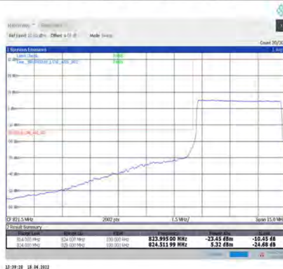
1-N5--15-5-L-6-CP-QPSK-Outer_Full-25@0-Ant1-seegraph-PASS-see graph
