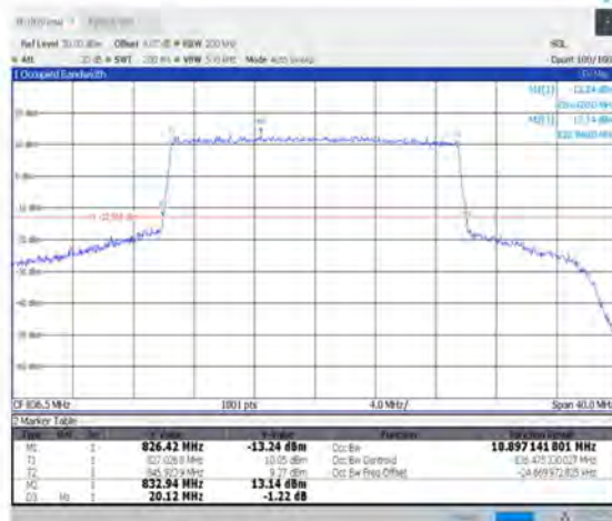
1-N5--15-20-M-8-CP-64QAM-Outer_Full-106@0- Ant1-18.897-20.120-≤20-PASS
