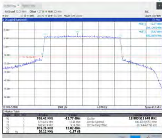
1-N5--15-20-M-7-CP-16QAM-Outer_Full-106@0- Ant1-18.884-20.120-≤20-PASS
