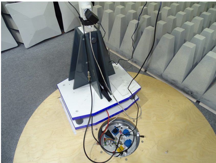
Photo 3: Test setup for radiated measurements
