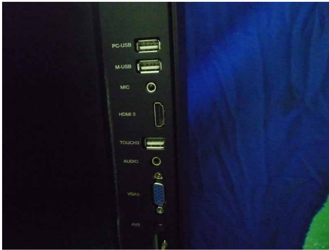
Figure 7 I/O Port of the EUT
