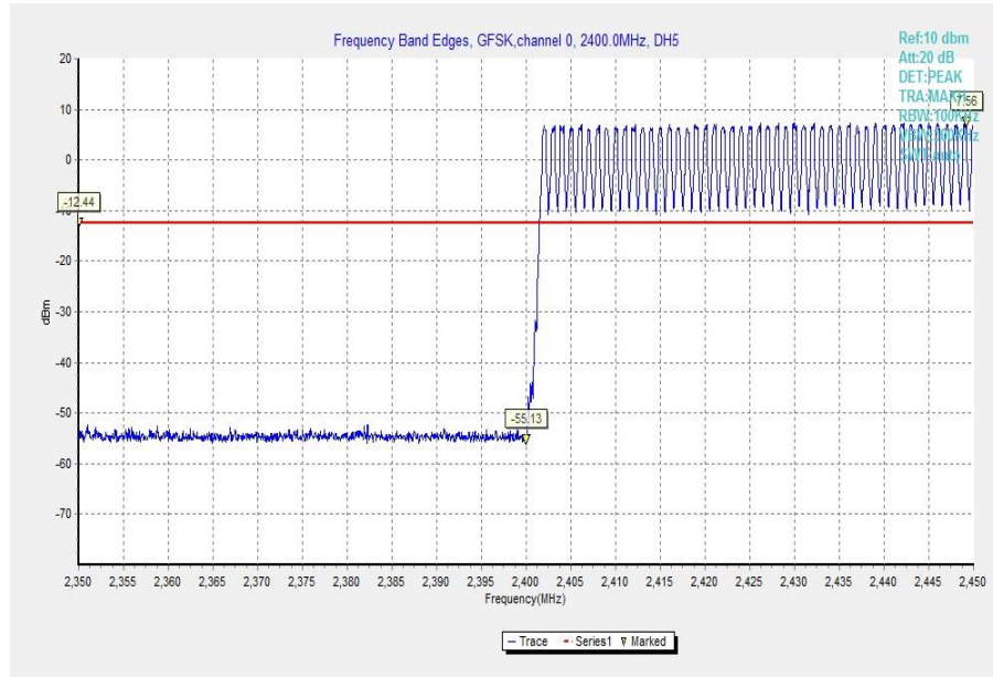
Fig. 10 Band Edges (GFSK, Ch 0, Hopping ON)
