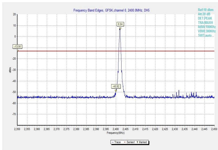
Fig. 16 Band Edges (GFSK, Ch 0, Hopping OFF)
