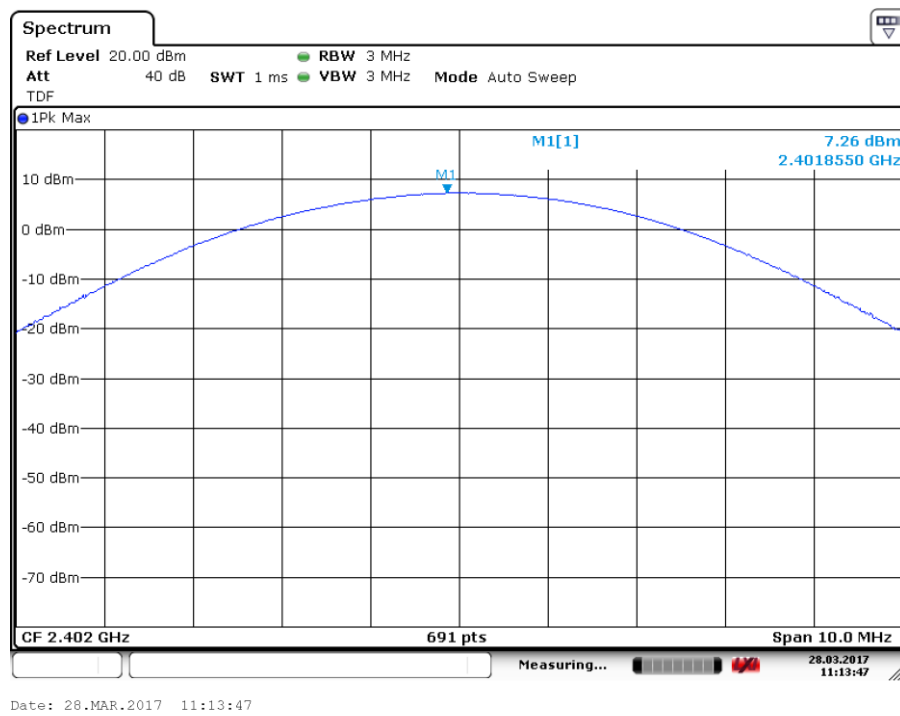
Fig. 7 Maximum Peak Output Power(8DPSK, Ch 0)
