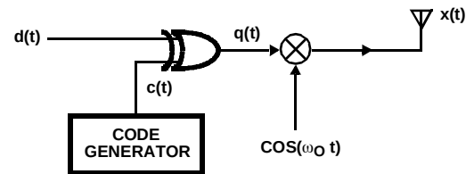
FIGURE 16. DSSS TRANSMITTER
