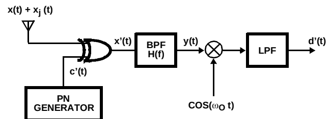
FIGURE 17. DSSS RECEIVER
