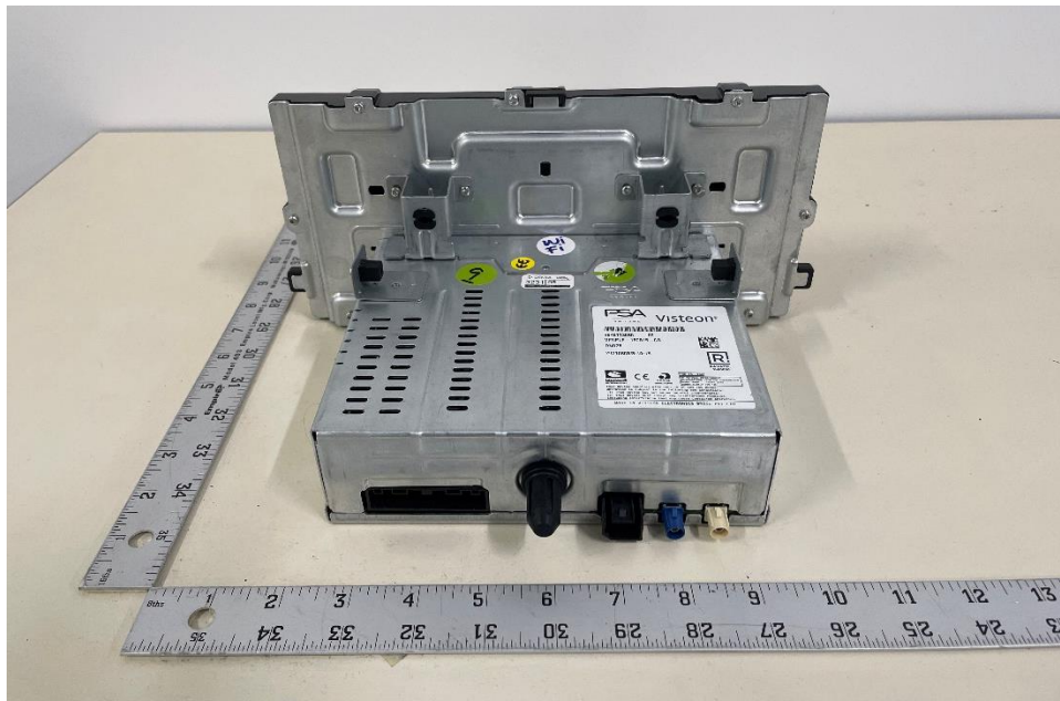
Figure B2: Rear view of the DUT
