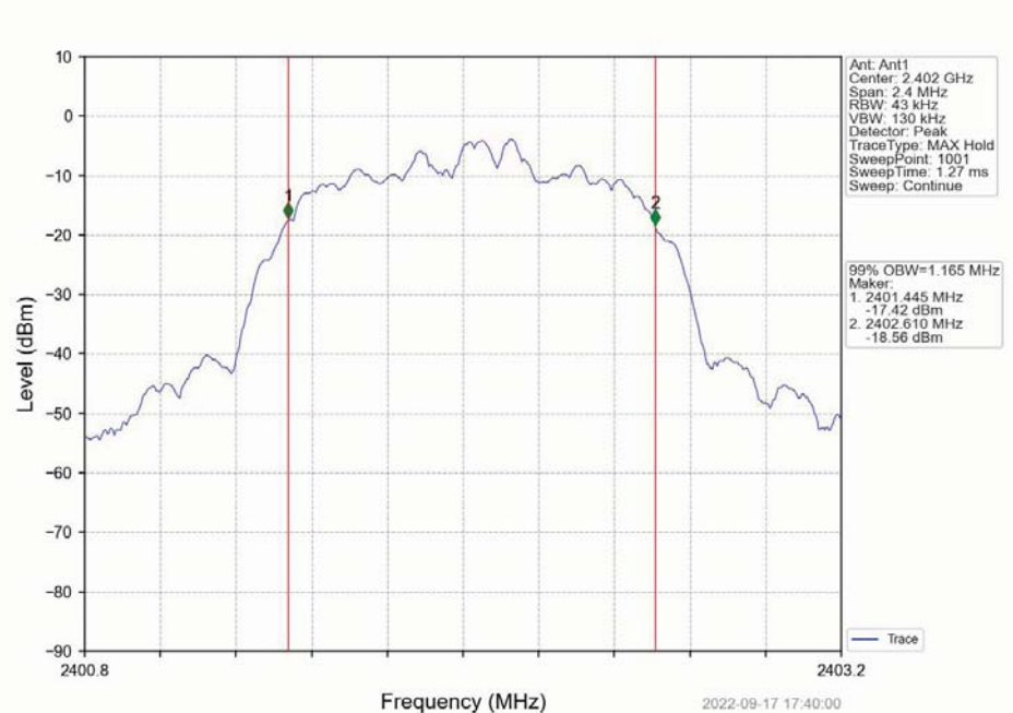
Pi/4DQPSK_2DH5_LCH_2402MHz_Ant1_NTNV
