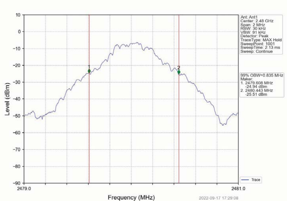
GFSK_DH5_HCH_2480MHz_Ant1_NTNV
