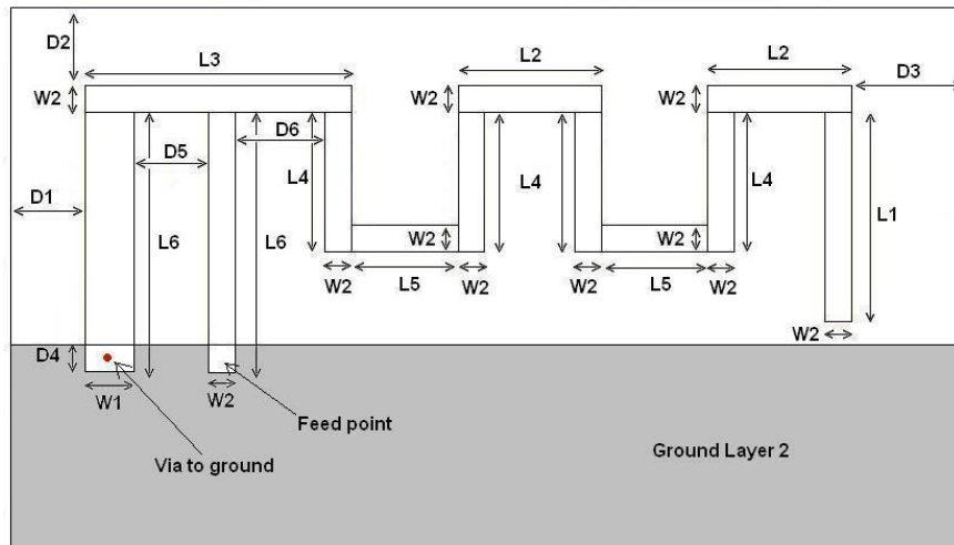
Figure 3: Antenna Dimensions
