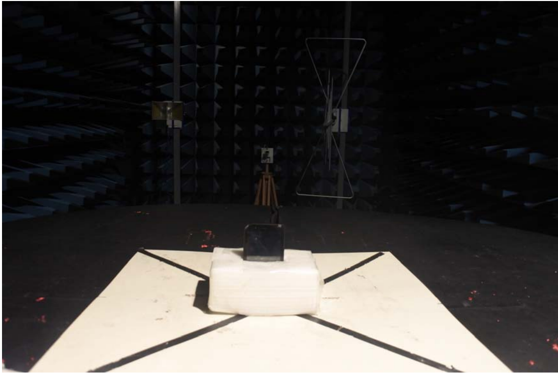
FCC Part15E Radiated Emission above 26.5-40GHz
