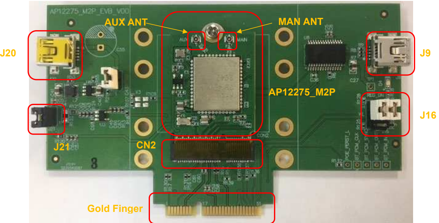
Figure7. Top view of WNFB-265AXI(BT) & AP12275_M2P EVB
