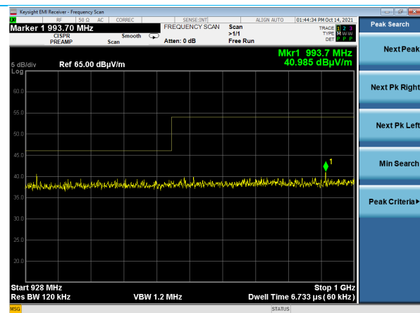
928-1000 MHz, Vertical Antenna Channel 10
