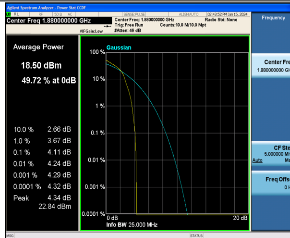
Band2-1.4MHz-16QAM-18900-1RB#0-PASS
