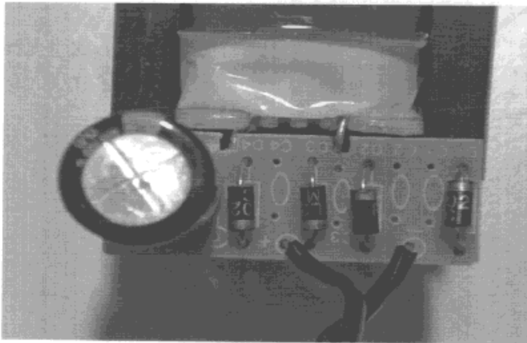
Inner View of Adaptor
