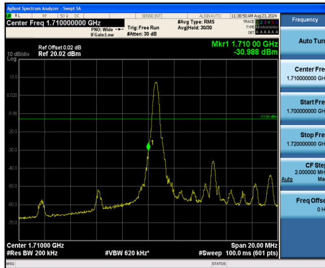
Band66-10MHz-16QAM-132022-1RB#49
