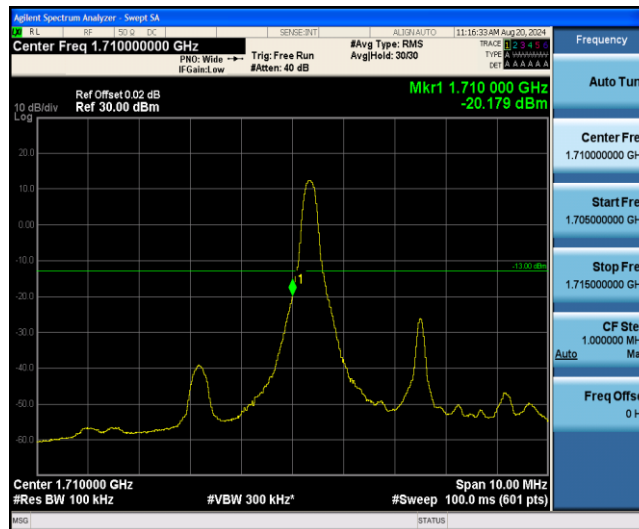
Band66-5MHz-QPSK-131997-1RB#24
