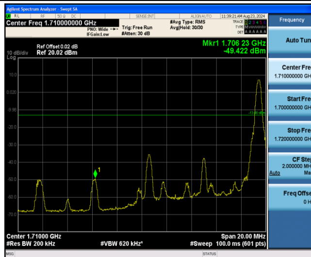
Band66-10MHz-16QAM-132022-27RB#0
