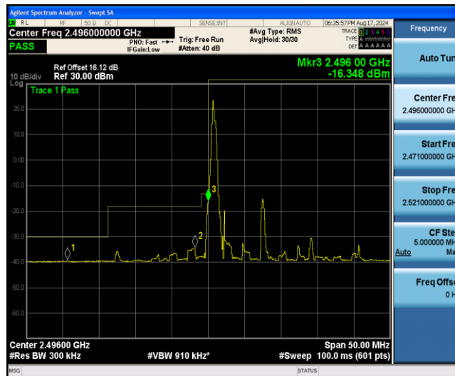
Band41-15MHz-16QAM-39725-27RB#0
