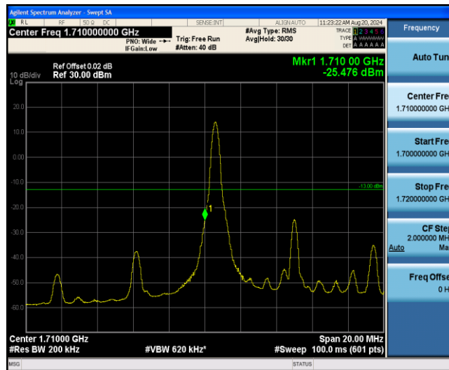
Band66-10MHz-QPSK-132022-1RB#49
