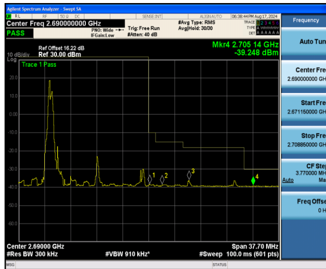
Band41-15MHz-16QAM-41515-27RB#0
