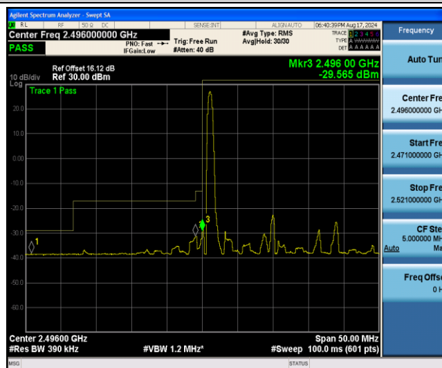
Band41-20MHz-16QAM-39750-27RB#0
