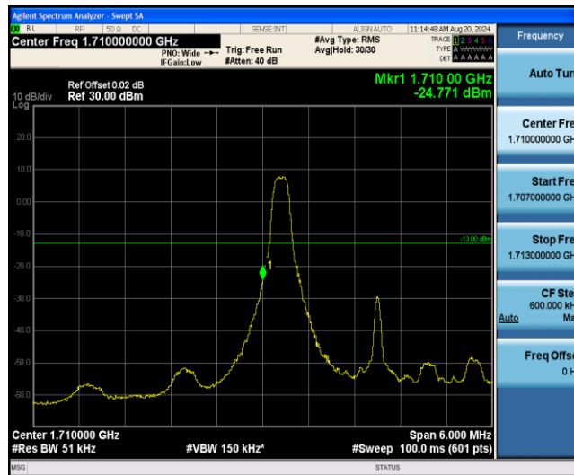
Band66-3MHz-16QAM-131987-1RB#14
