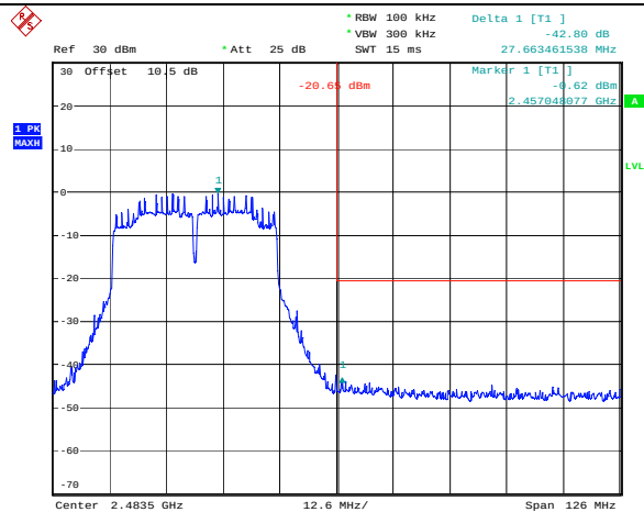
802.11n ht40_Chain 0_Highest Band edge
