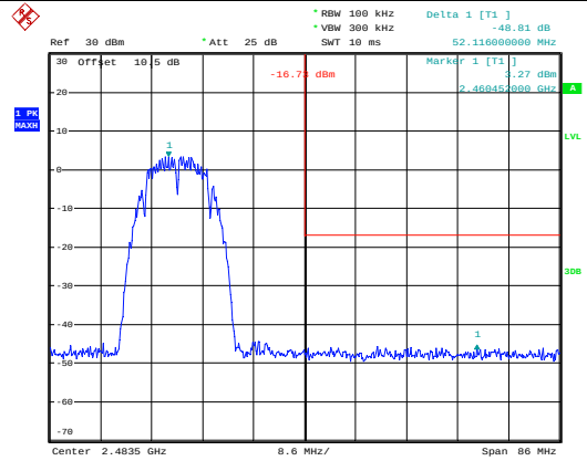
802.11b_Chain 0_Highest Band edge
