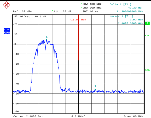
802.11b_Chain 1_Highest Band edge
