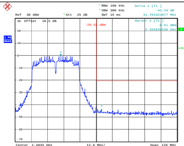
802.11n ht40_Chain 1_Highest Band edge
