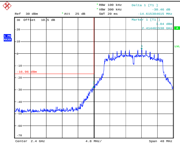
802.11n ht20_Chain 1_Lowest Band edge
