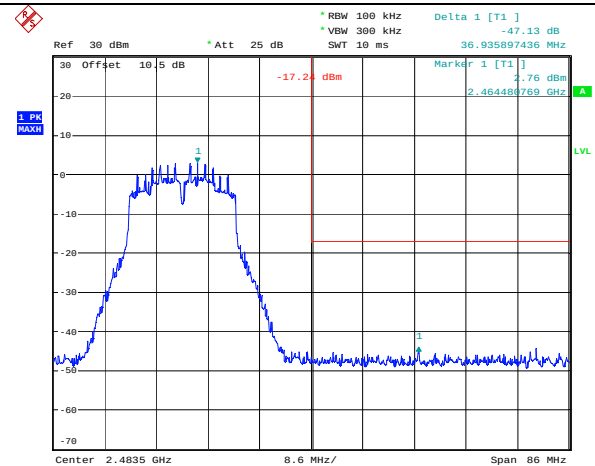
802.11n ht20_Chain 1_Highest Band edge
