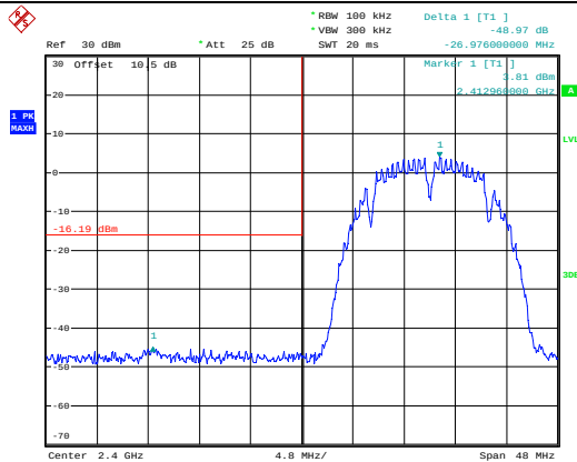
802.11b_Chain 1_Lowest Band edge
