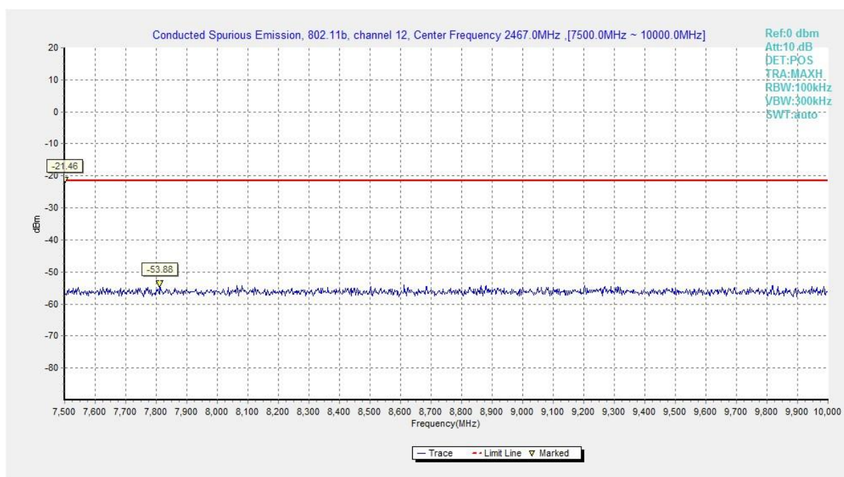
Fig.A.6.1.29 Conducted Spurious Emission (802.11b, Ch12, 7.5 GHz-10 GHz)
