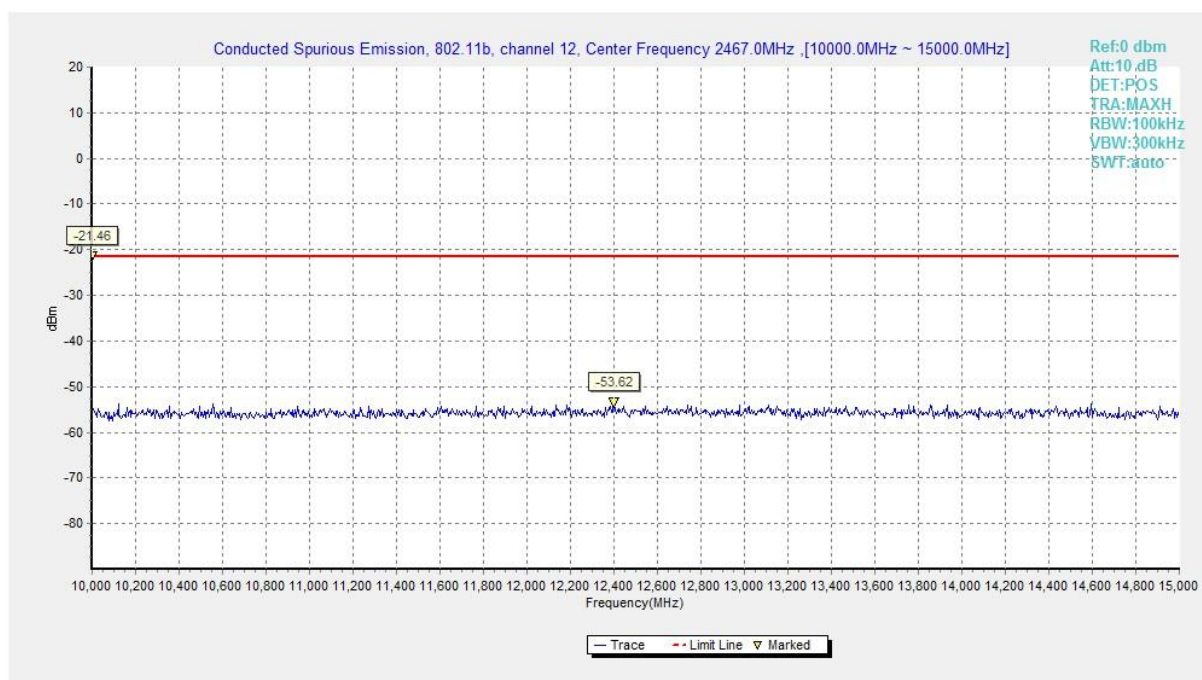
Fig.A.6.1.30 Conducted Spurious Emission (802.11b, Ch12, 10 GHz-15 GHz)
