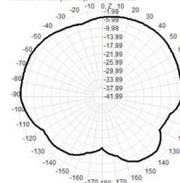
900.0MHz Total(E2-YZ), Max=-2.23dBi
