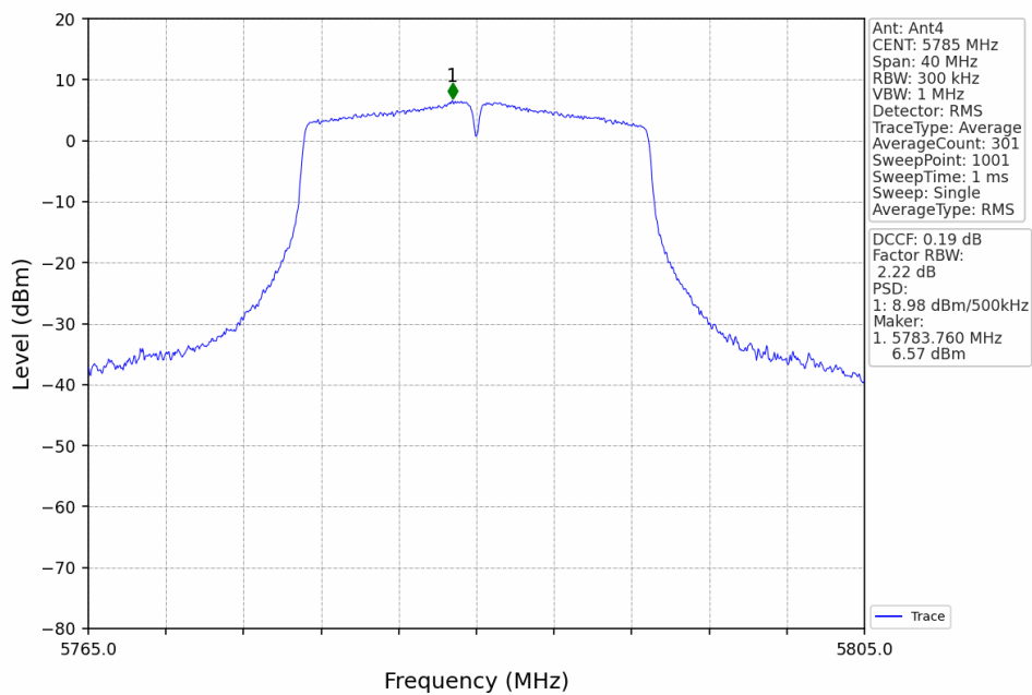
802.11n(HT20)_MCH_5785MHz_Ant4_NTNV
