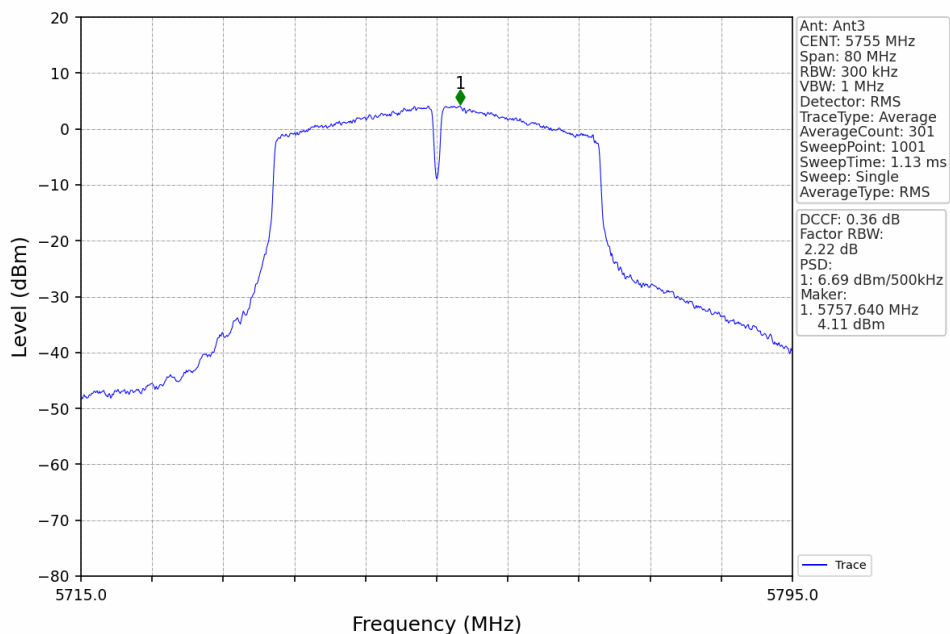
802.11ac(VHT40)_LCH_5755MHz_Ant3_NTNV
