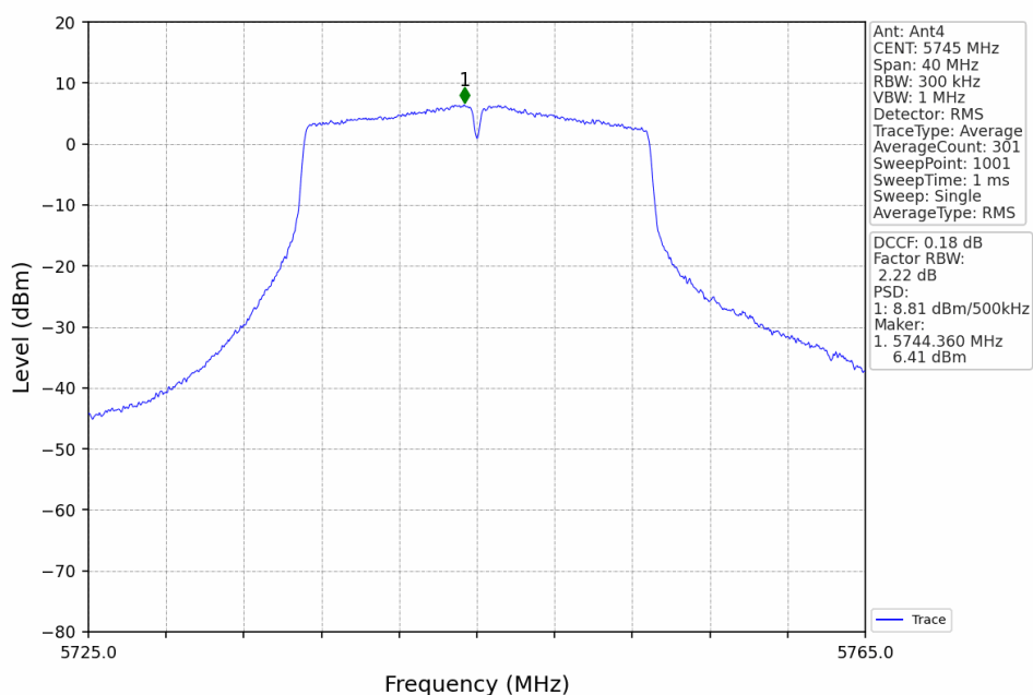
802.11ac(VHT20)_LCH_5745MHz_Ant4_NTNV
