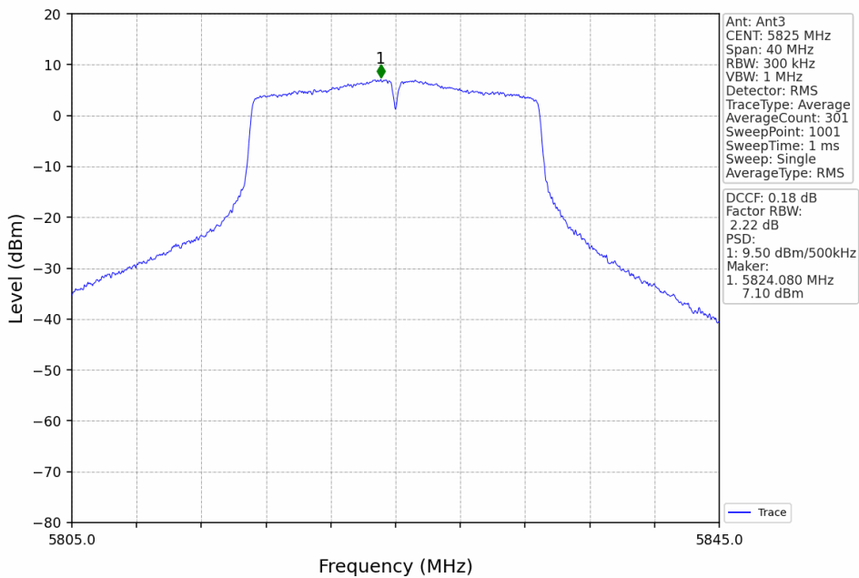
802.11n(HT20)_HCH_5825MHz_Ant3_NTNV
