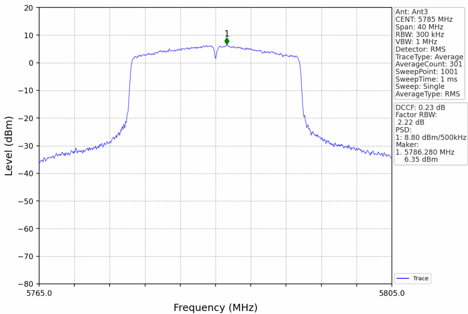
802.11ax(HEW20)_MCH_5785MHz_RU242_Left_Ant3_NTNV
