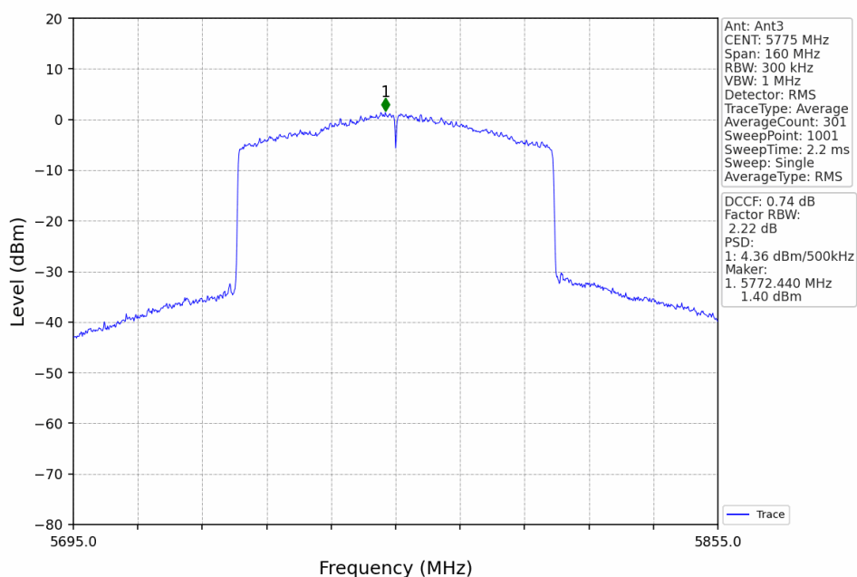
802.11ax(HEW80)_MCH_5775MHz_RU996_Left_Ant3_NTNV
