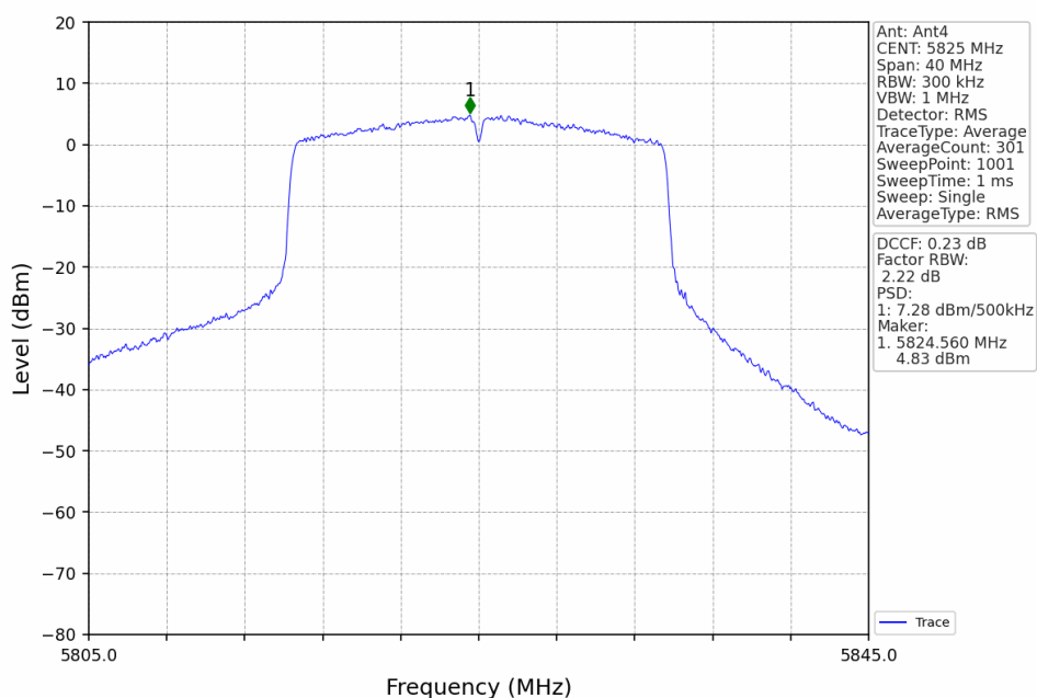
802.11ax(HEW20)_HCH_5825MHz_RU242_Left_Ant4_NTNV
