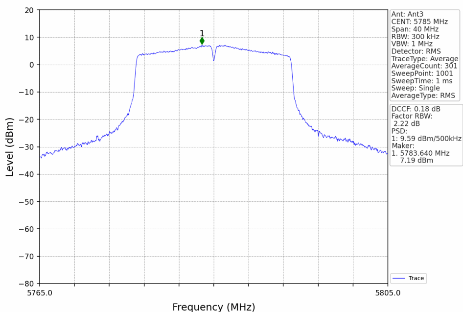
802.11ac(VHT20)_MCH_5785MHz_Ant3_NTNV
