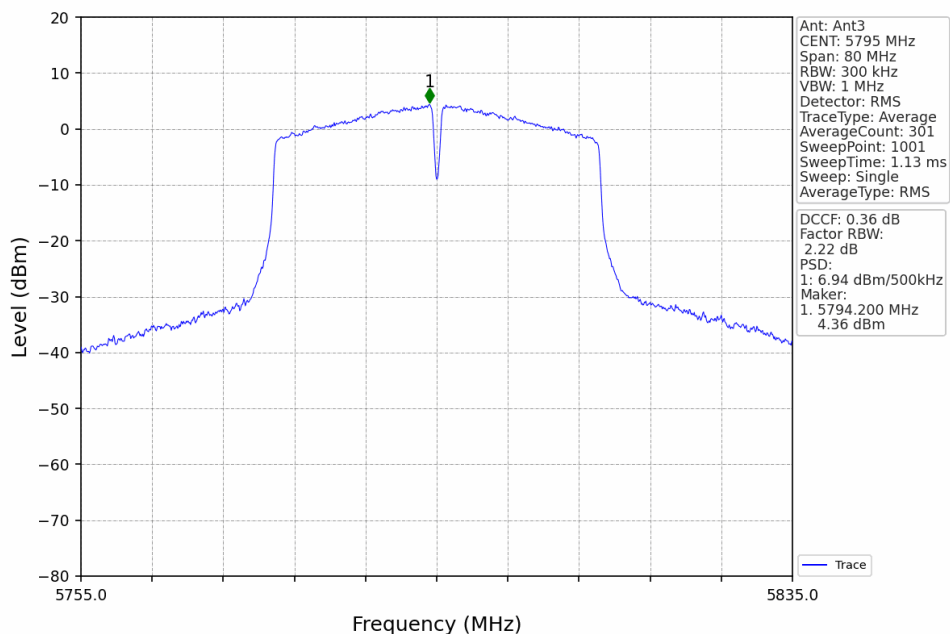
802.11n(HT40)_HCH_5795MHz_Ant3_NTNV
