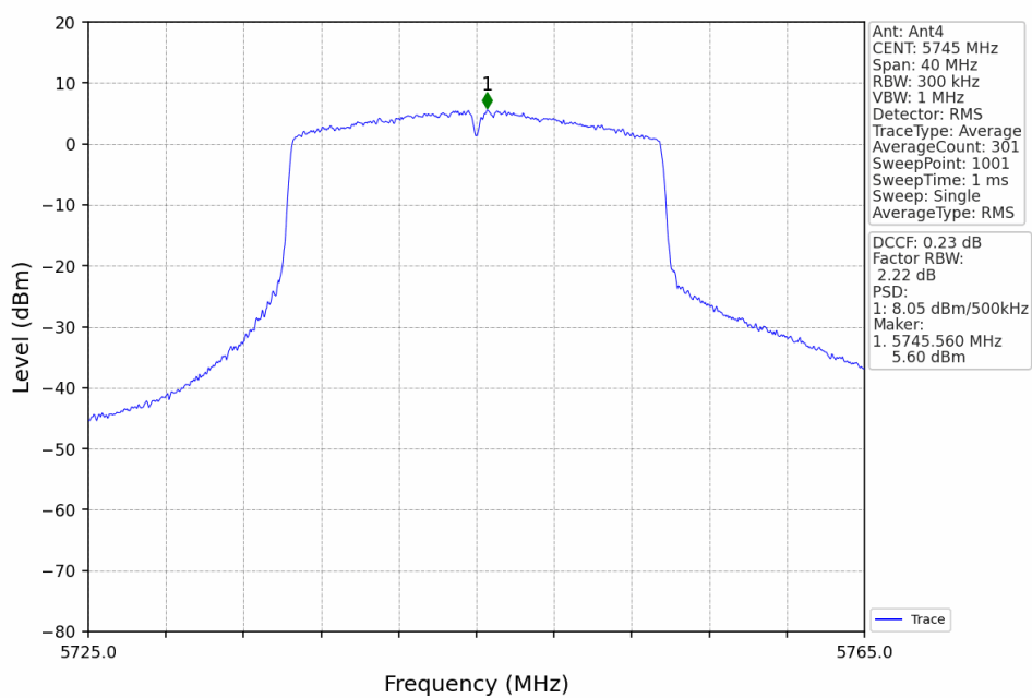
802.11ax(HEW20)_LCH_5745MHz_RU242_Left_Ant4_NTNV
