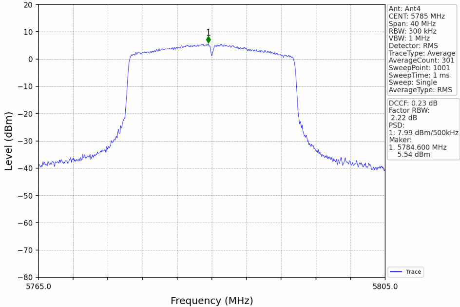
802.11ax(HEW20)_MCH_5785MHz_RU242_Left_MIMO_NTNV
