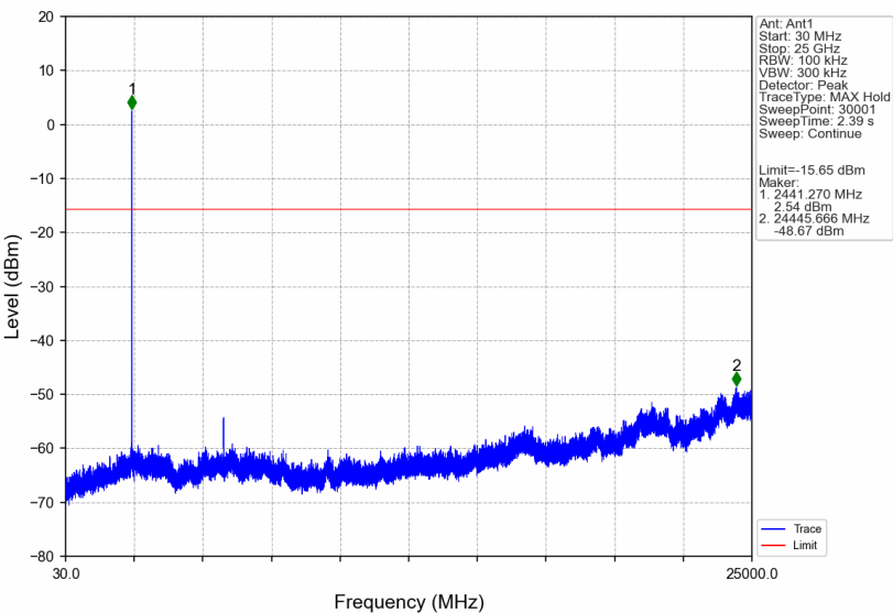
Pi/4DQPSK_2DH5_MCH_2441MHz_Ant1_NTNV
